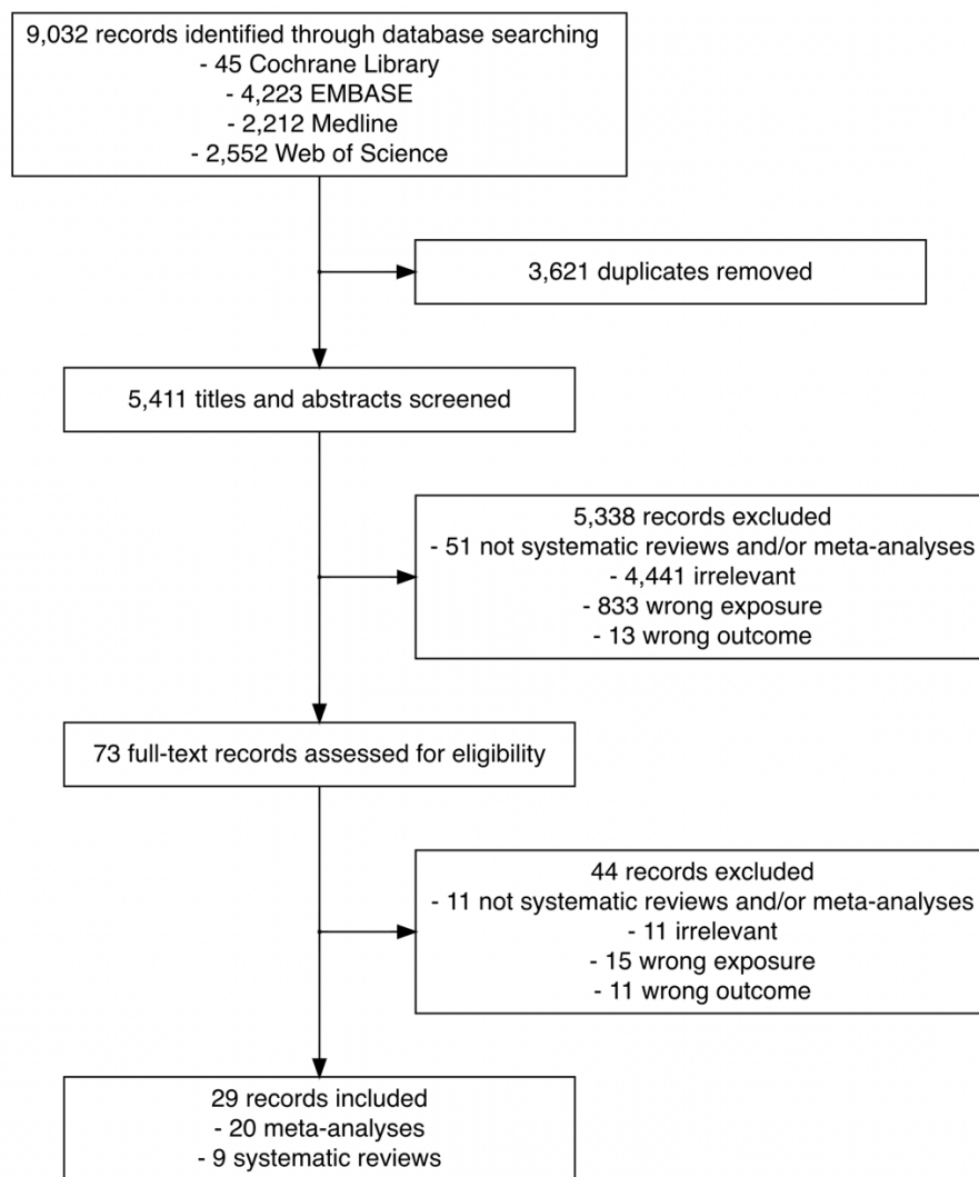
Figure 1. Flowchart of the search and study selection of systematic reviews and meta-analyses on the association between time to cancer diagnosis and/or treatment and clinical outcomes
