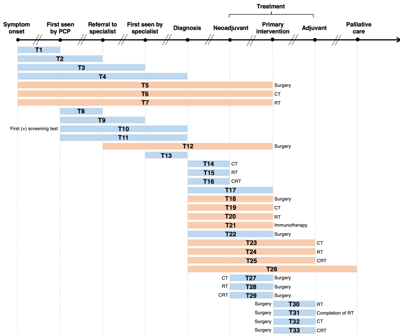
Figure 2. Visualization of lag time intervals identified in systematic reviews and/or meta-analyses on the association between time to cancer diagnosis and/or treatment and clinical outcomes
