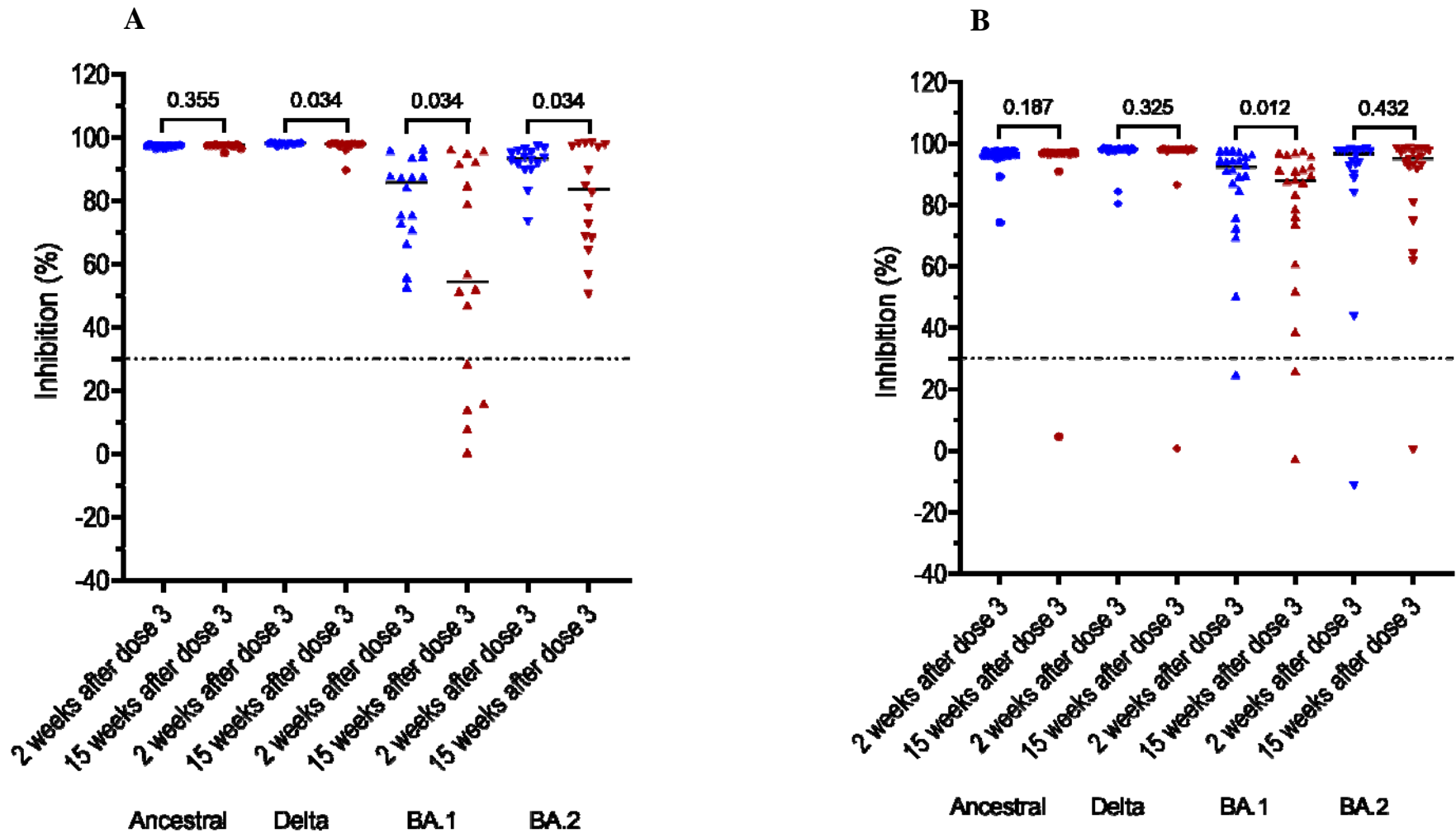
Figure 3: Persistence of neutralising antibodies at month 3 after the booster dose in those without documented breakthrough infection after the booster dose, A ) participants of G1, and B ) participants of G2. Horizontal dot lines indicate assay cut-off, Numbers indicates p values.
