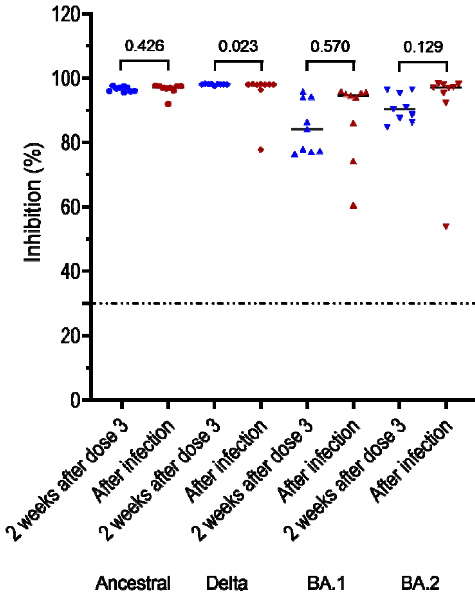
Supplementary Figure 1: Neutralising antibodies measured at week 2 and 15 after booster vaccination in 11 HCWs with an infection episode documented after the booster dose
