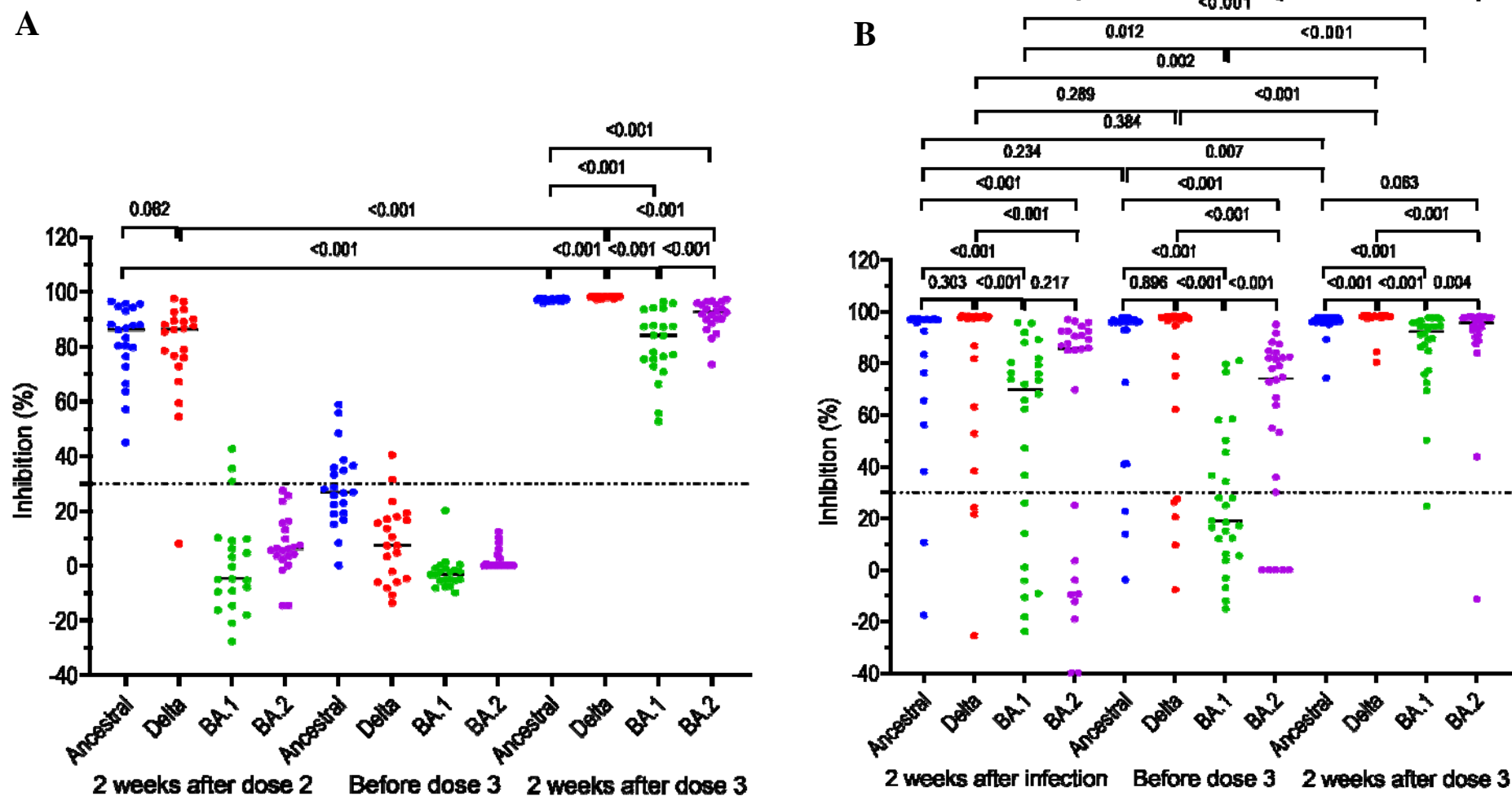
Figure 2: Neutralizing antibodies against SARS-CoV-2 ancestral strain and VOCs (Delta, BA.1 and BA.2) in individuals with and without prior breakthrough Delta variant infection measured at different time points prior to booster vaccination and at week 2 post booster dose. Horizontal dot lines indicate assay cut-off. Numbers indicates p values.
