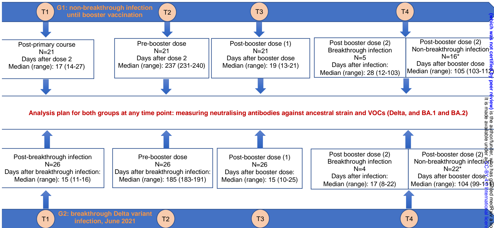
Figure 1: Illustration showing the distribution of the study participants and sampling schedules for neutralising antibody measurement Note to Figure 1: *after excluding cases with a SARS-CoV-2 infection episode recorded after the booster dose.
