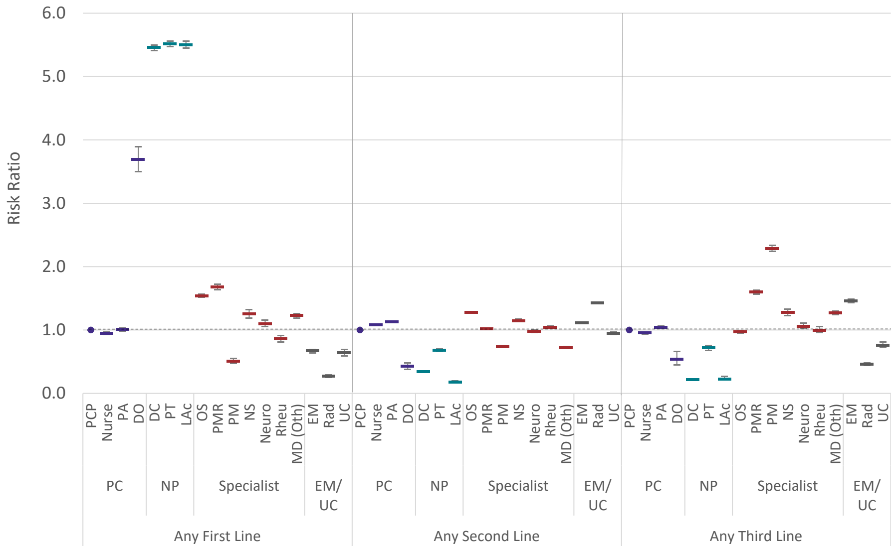
Figure 3 - Risk ratio and 95% confidence interval for non-surgical low back pain episodic service exposure by initial contact health care provider compared to PCP reference. PC=Primary Care, NP=Non-Prescriber, EM/UC=Emergency Medicine/Urgent Care, PCP=Primary Care Provider; PA=Physician Assistant; DO=Doctor of Osteopathy; DC=Doctor of Chiropractic; PT=Physical Therapist; Lac=Licensed Acupuncturist; OS=Orthopedic Surgeon; PMR=Physical Medicine and Rehabilitation; PM=Pain Management, NS=Neurosurgeon; Neuro=Neurologist; Rheum=Rheumatologist; MD (Oth)=Other medical physician specialties, EM=Emergency Medicine; Rad=Radiologist; UC=Urgent Care
