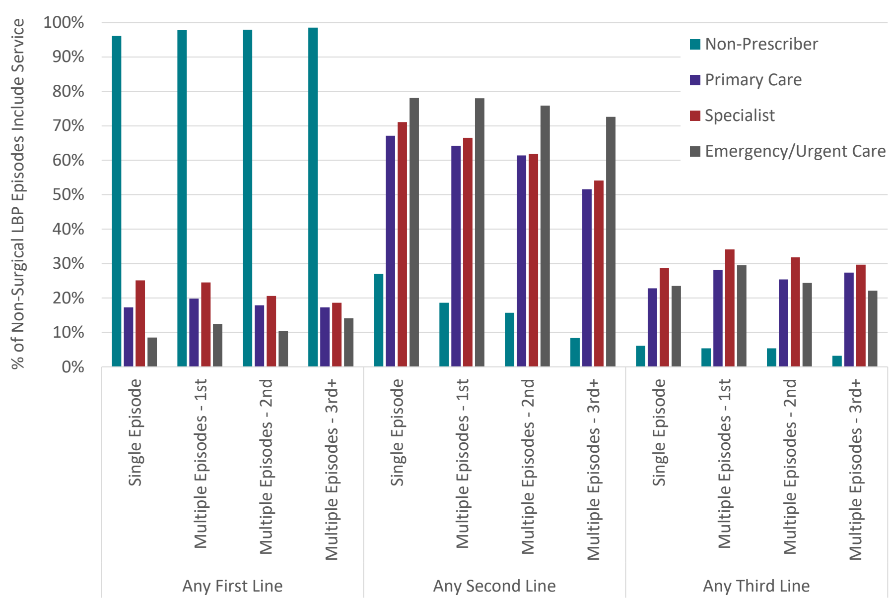
Figure 4. Percent of low back pain episodes including any first-, second- or third-line service by episode sequence cohort and type of initial contact health care provider
