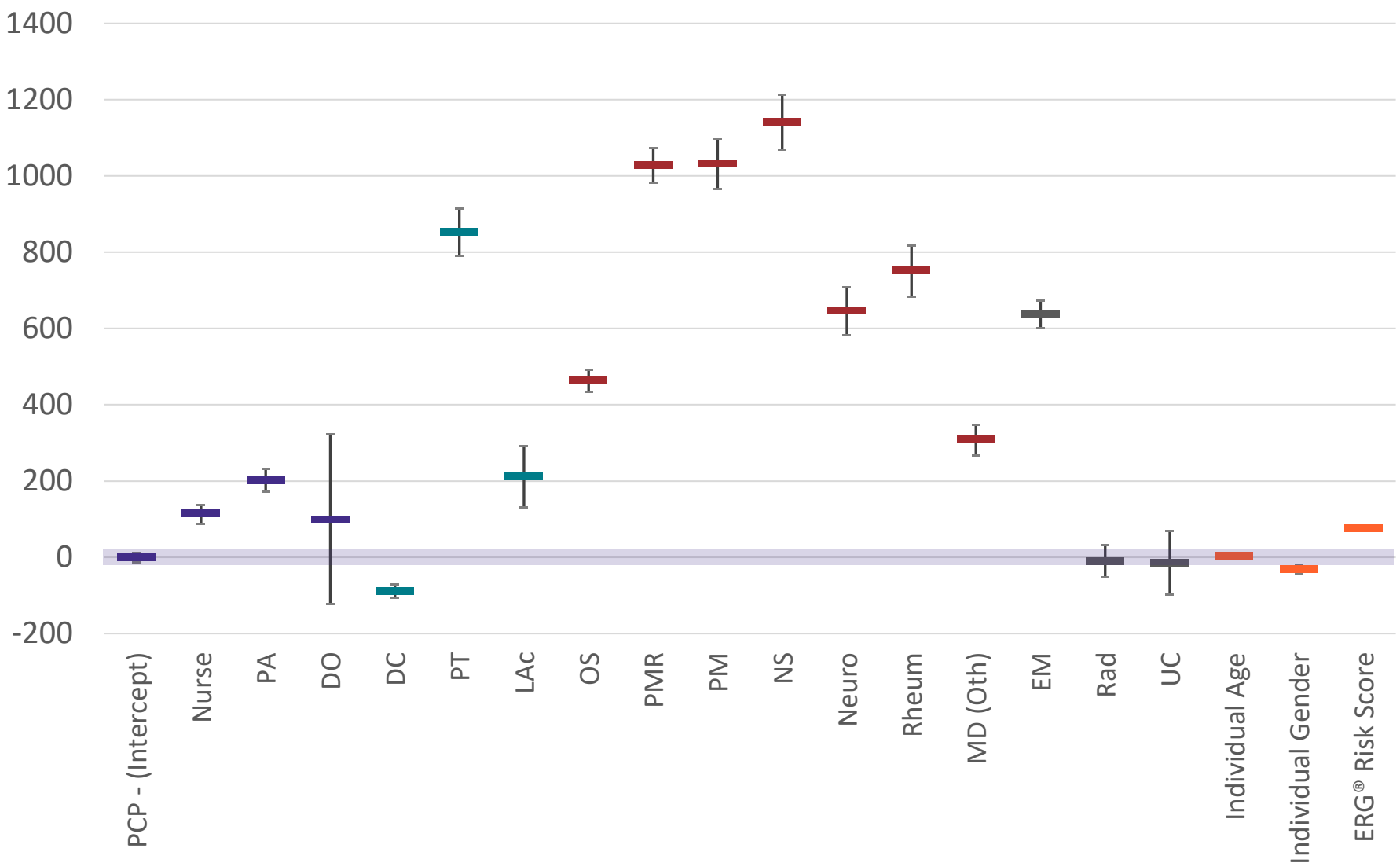
Figure 5. Low back pain non-surgical total episode cost regression estimates and 95% confidence intervals by type of initial contact HCP (0 Intercept = PCP reference group). PCP=Primary Care Provider; PA=Physician Assistant; DO=Doctor of Osteopathy; DC=Doctor of Chiropractic; PT=Physical Therapist; LAC=Licensed Acupuncturist; OS=Orthopedic Surgeon; PMR=Physical Medicine and Rehabilitation; PM=Pain Management, NS=Neurosurgeon; Neuro=Neurologist; Rheum=Rheumatologist; MD (Oth)=Other medical physician specialties, EM=Emergency Medicine; Rad=Radiologist; UC=Urgent Care
