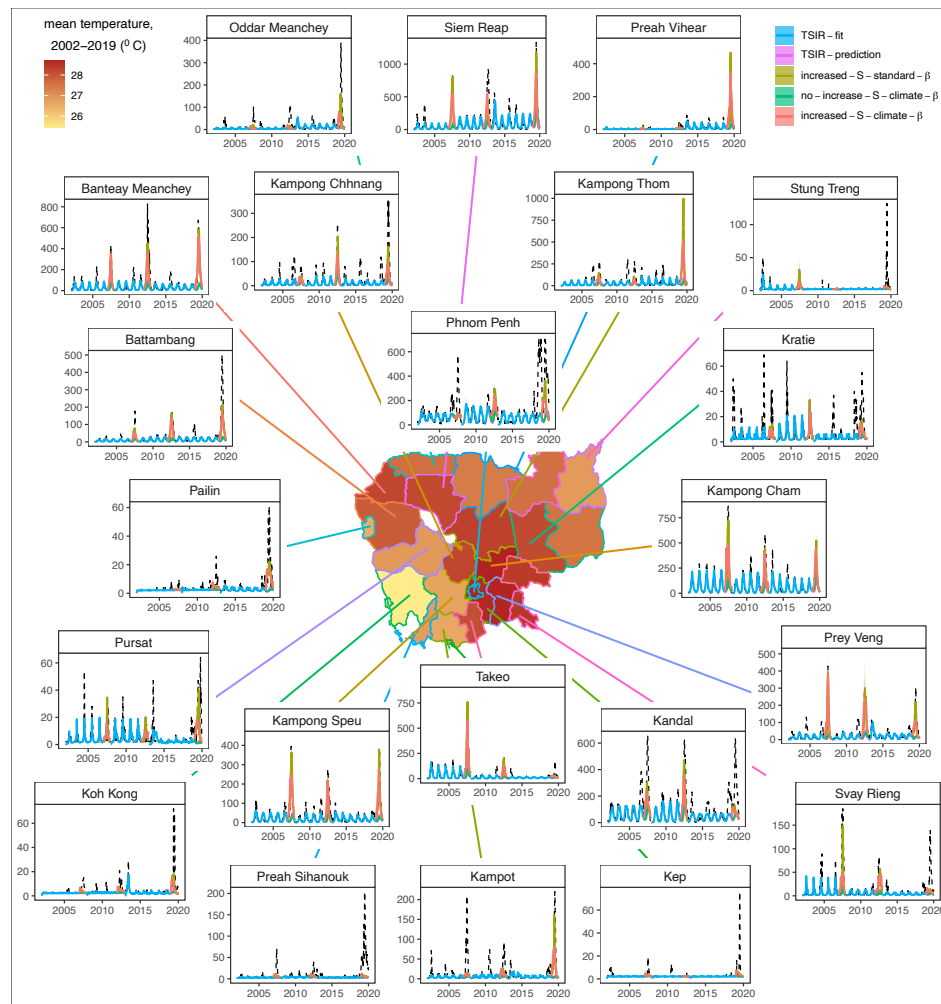
250 Figure 1. Climate-informed TSIR insights into epidemic dynamics of DENV in Cambodia. Inset panels 251 show province level clinicosyndromic reported DENV cases ( dashed black lines ) with fitted TSIR output to 252 the three inter-epidemic periods (2002-2006, 2008-2011, 2013-2018; blue lines ) and TSIR projections for 253 epidemic years (2007, 2012, 2019) under trained biweekly transmission rate ( \beta ) estimates ( pink lines ), 254 incorporating a factorial increase in the susceptible population ( gold lines ), using a climate-projected \beta 255 estimated from lagged temperature and precipitation data by province ( green lines ), or using both climate- 256 projected \beta and a factorial increase in the susceptible population ( red lines ) ( SI Appendix , Table S2, S5). 257 The center map shows province level administrative boundaries for Cambodia, shaded by the mean 258 biweekly temperature in 2020.
