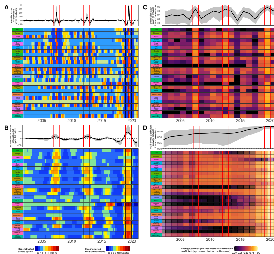
Figure 2. Wavelet reconstructions show heightened synchrony in epidemic years. Reconstructed A
