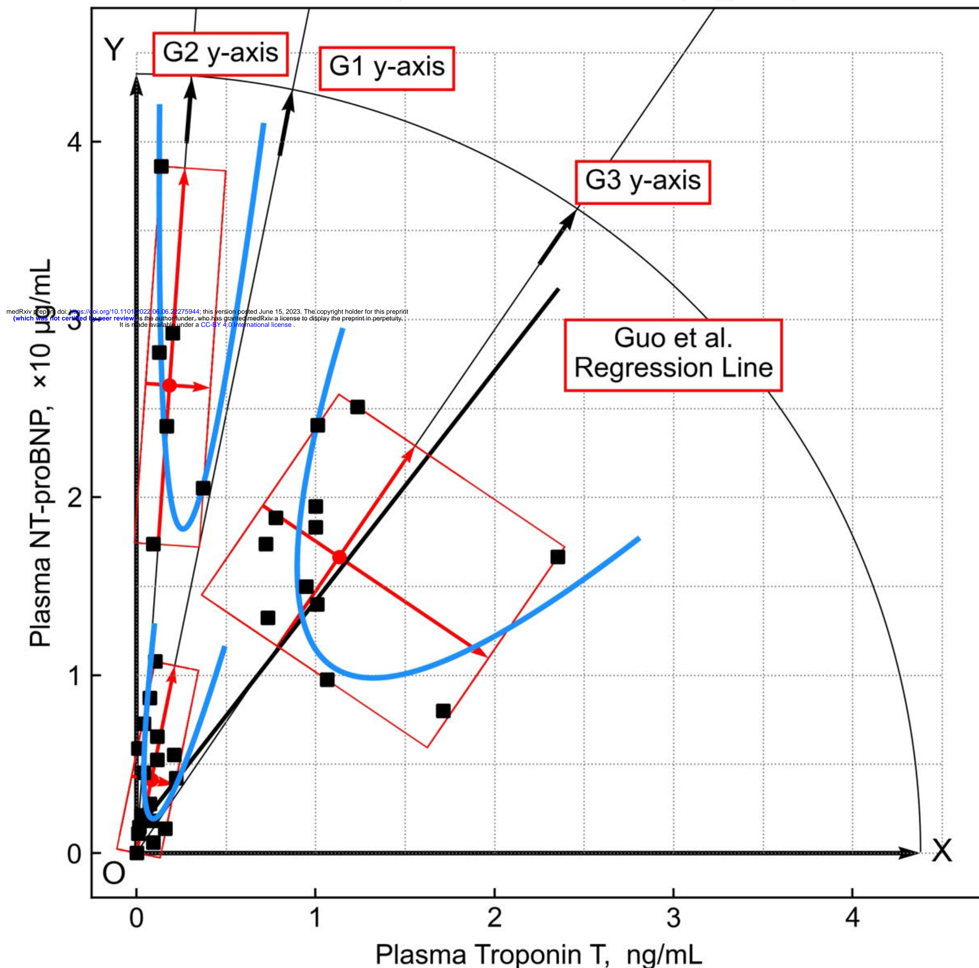
Re-analysis Guo et al. 2020 (Fig. 1B)
