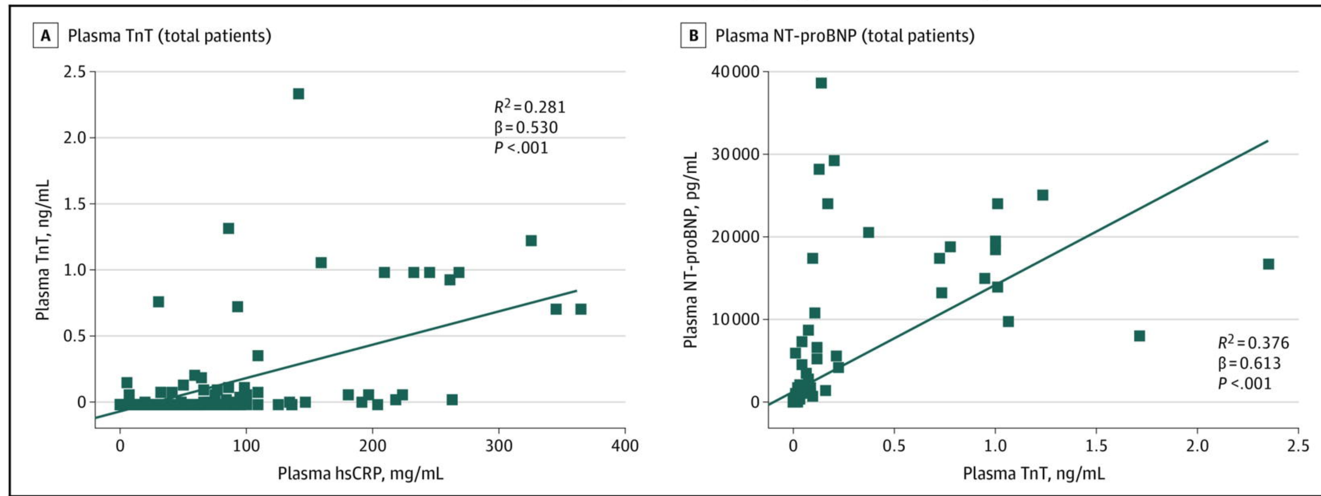
Re-analysis Guo et al. 2020 (Fig. 1B)
