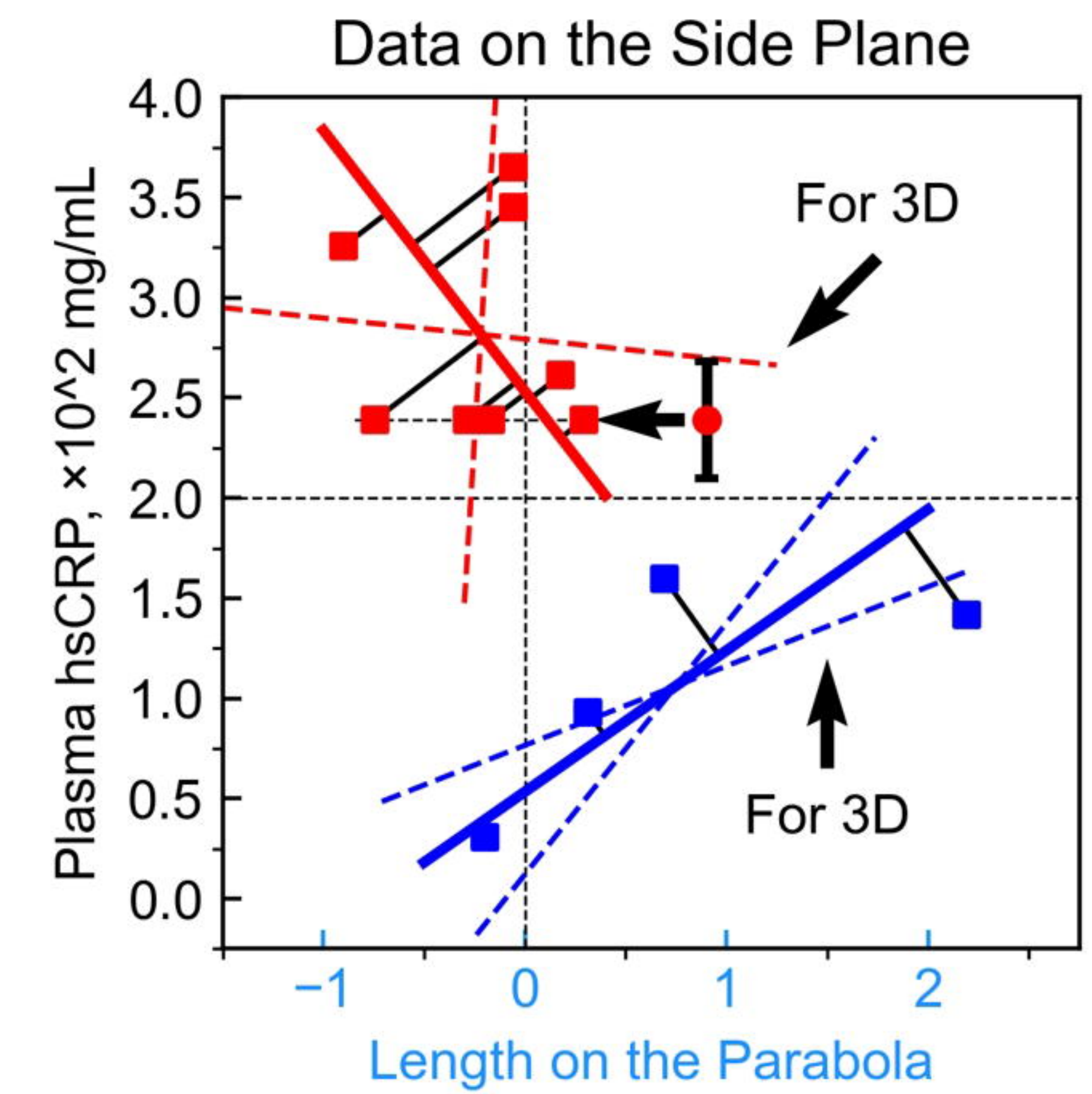
3D Data Visualization on the Plane of Guo et al. Fig. 1B (Sub-group 3)
