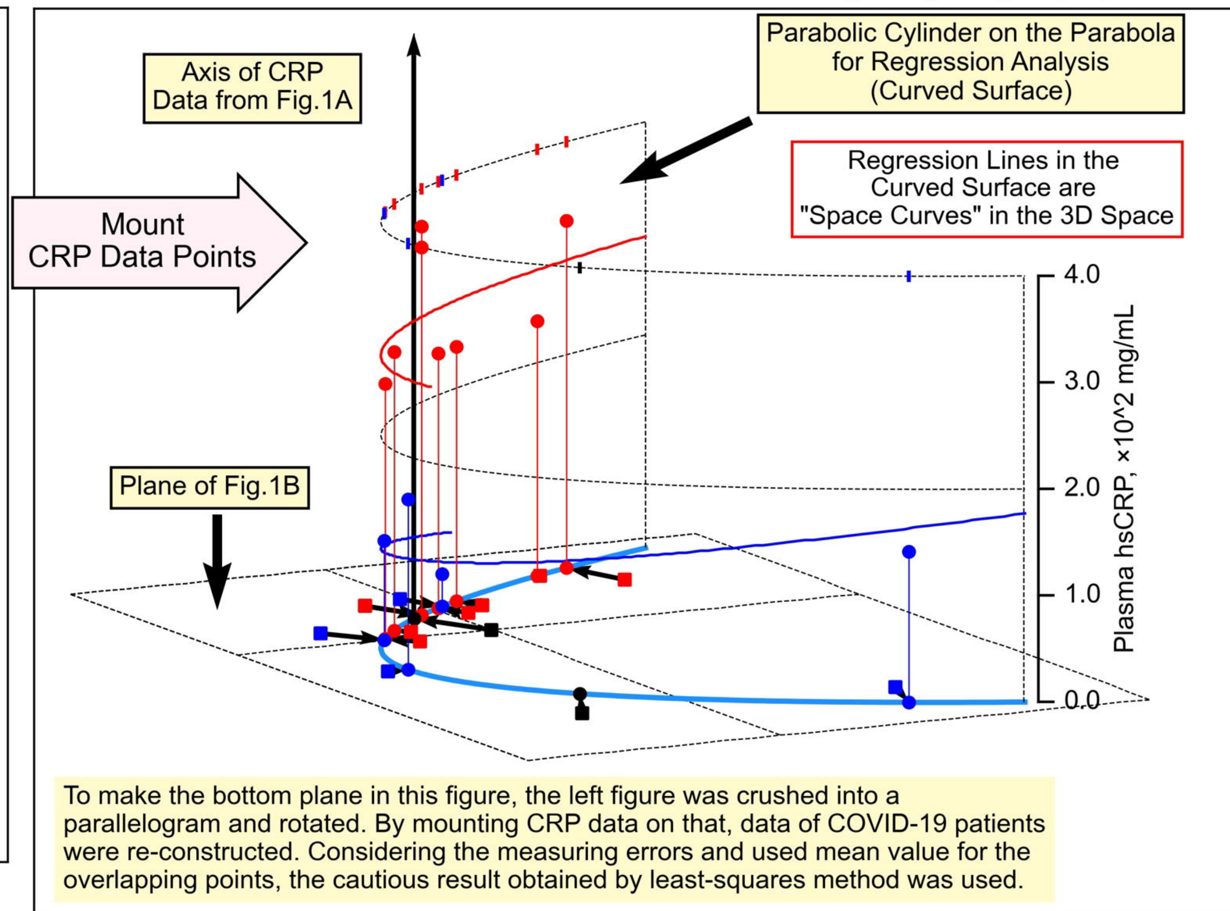
3D Data Visualization on the Plane of Guo et al. Fig. 1B (Sub-group 3)
