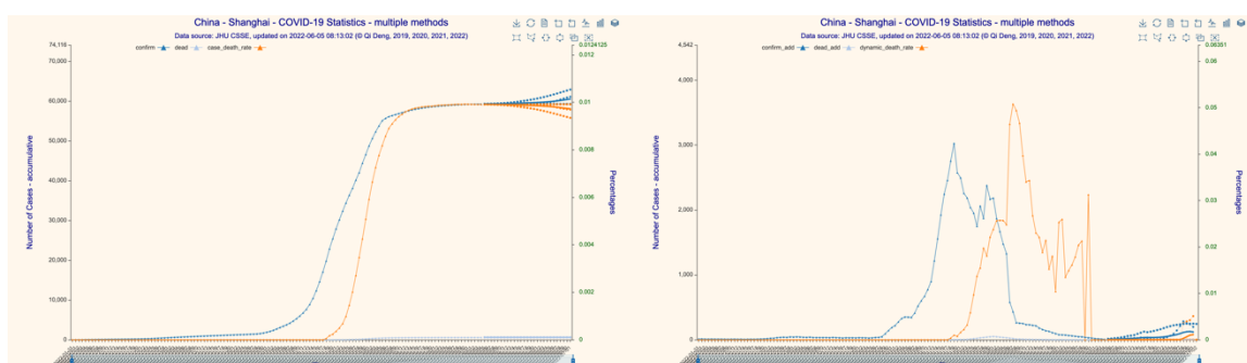
Fig. 3. 28-day forecast for confirmed/deceased cases in Shanghai
