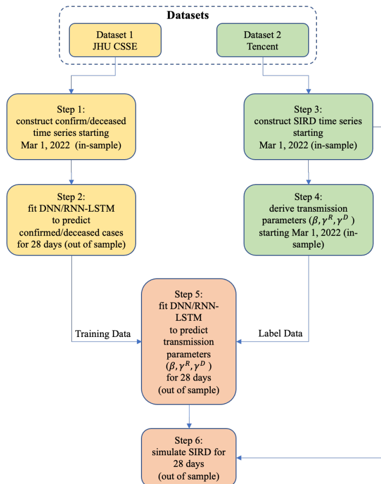
Fig. 1. The methodology flowchart
