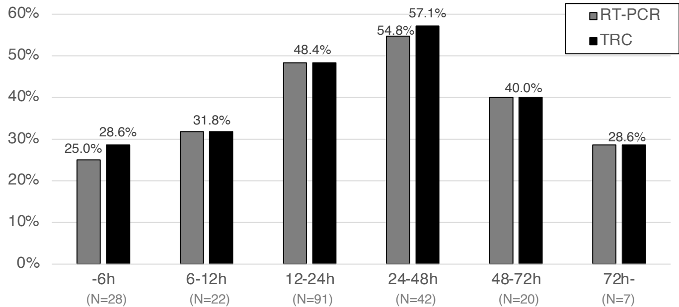
Figure 2. Positive rate of influenza in each test by time since onset of symptoms
