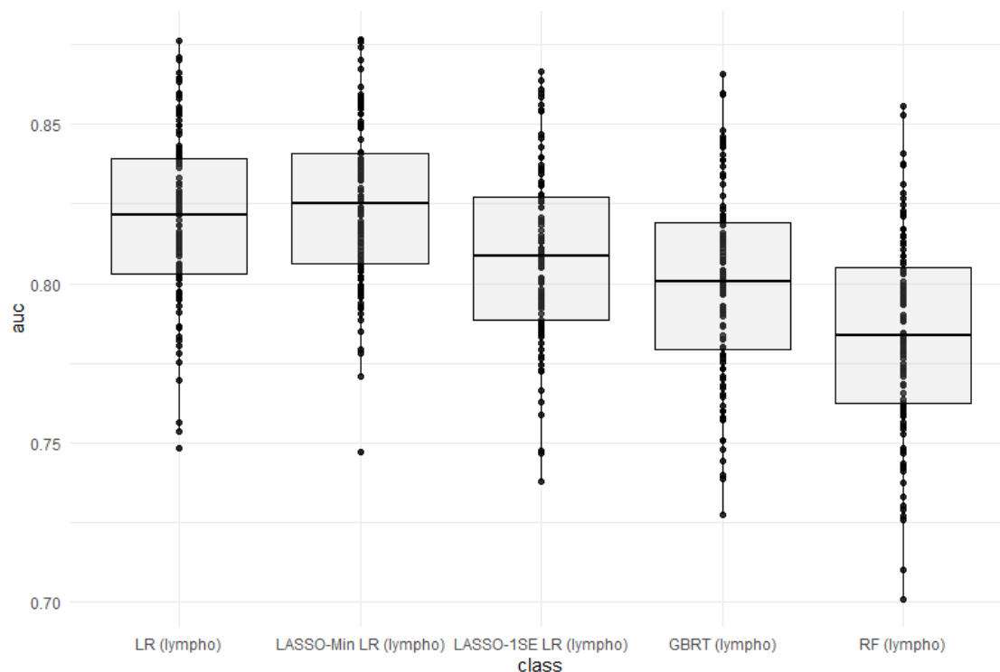
Figure 2. Predictive performance of the developed models (AUC) in internal validation. LR - logistic regression, LASSO-Min LR - least absolute shrinkage and selection operator regularized logistic regression with lambda hyperparameter optimized to yield minimum mean squared error within an inner 5-fold cross validation in the training set. LASSO-1SE - least absolute shrinkage and selection operator regularized logistic regression with lambda hyperparameter increased from lambda-min, so that mean squared error stays within one standard error within an inner 5-fold cross validation in the training set. GBRT - gradient boosted regression trees. RF - random forest. lympho – including lymphocyte count as predictor variable.
