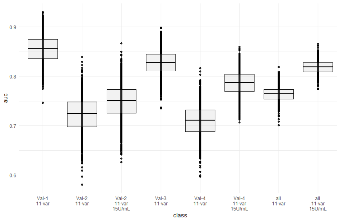
Figure 3. Predictive performance (AUC-ROC) of the 11-variable model in external validation.
