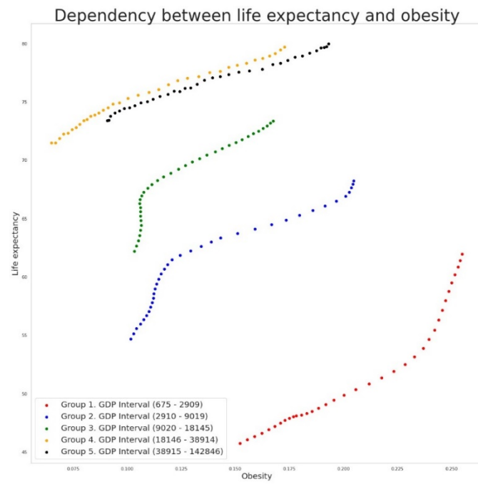
The relationship between LEB and prevalence of obesity, countries grouped by GDP PC 2013. Ordinate: LEB, years. Abscissa: Obesity prevalence, %.
