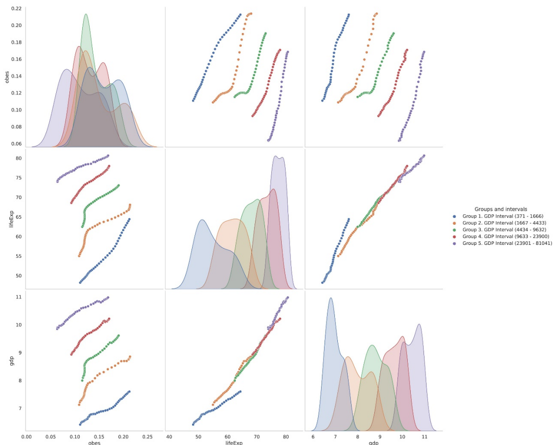
Figure 3: Double chart, grouping of countries by GDP PC 1997. Abscissa: obesity prevalence, %; LEB, years; GDP PC. Ordinate: GDP PC; LEB, years; obesity prevalence (bottom to up). Note log scale for GDP PC
