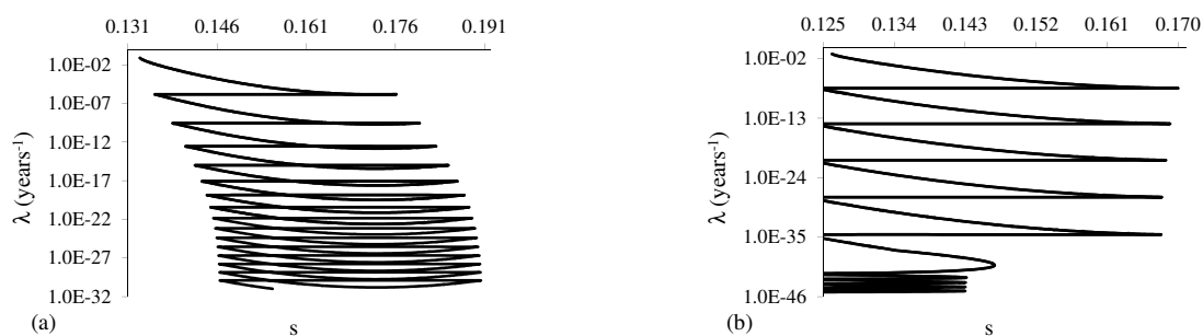
Figure 16: Phase space portrait (from 0 to 50 years ) for: (a) p = 23\% , with s oscillating beyond the equilibrium value, and (b) p = 27\% , with s oscillating below the equilibrium value.
