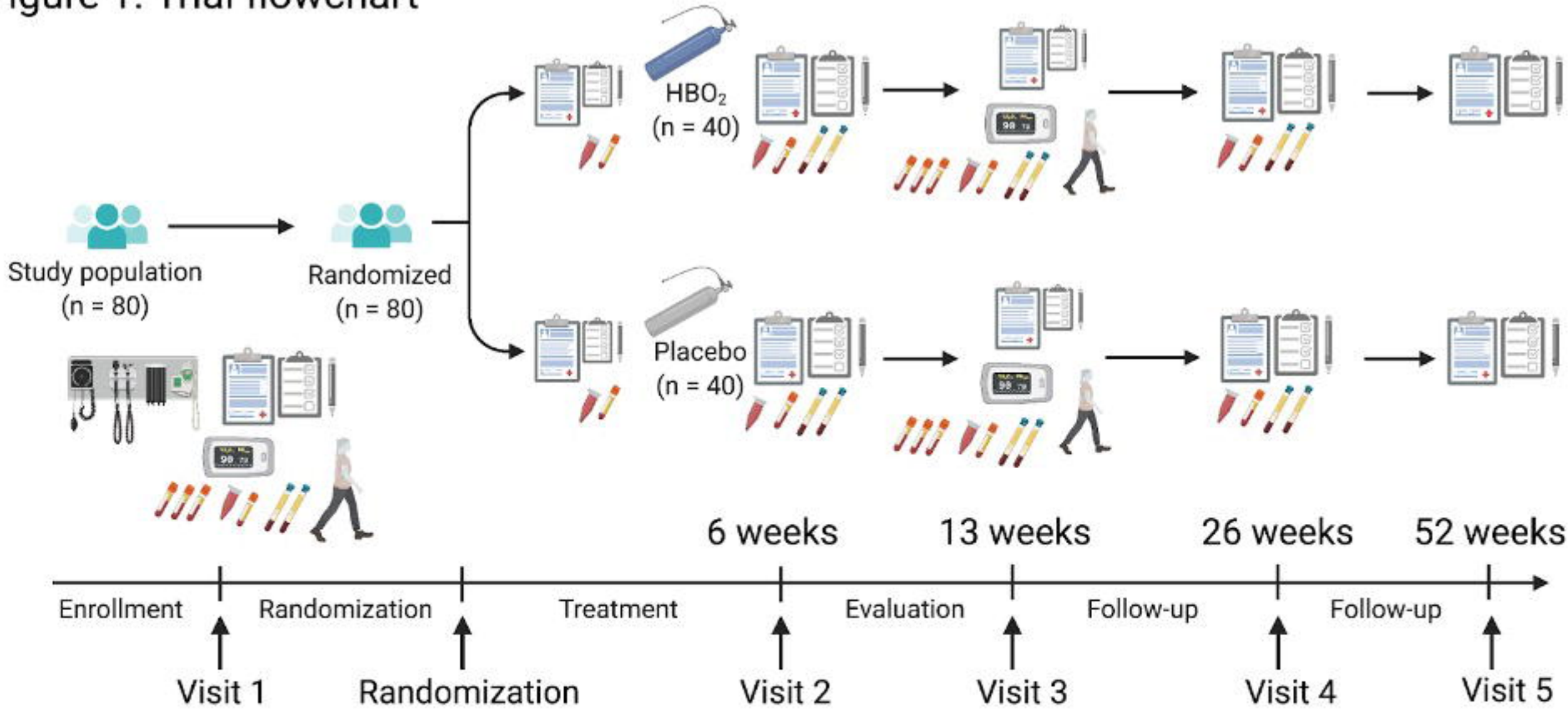
Figure 1. Trial flowchart
