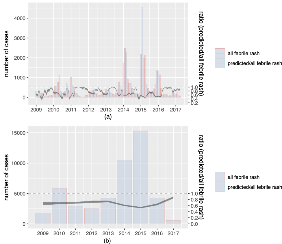
Figure 6: Ratio between predicted and suspected cases aligned with number of suspected cases, aggregated by (a) month and (b) year
