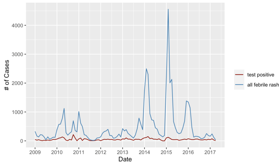
Figure 2: The aggregated number of confirmed cases and suspected cases from 2009 to 2017 in Ethiopia
