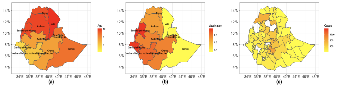
Figure 1: Distributions of (a) mean age at province level (b) mean number of vaccination received at province level and (c) number of cases at district level of all records with IgM test status on map of Ethiopia
