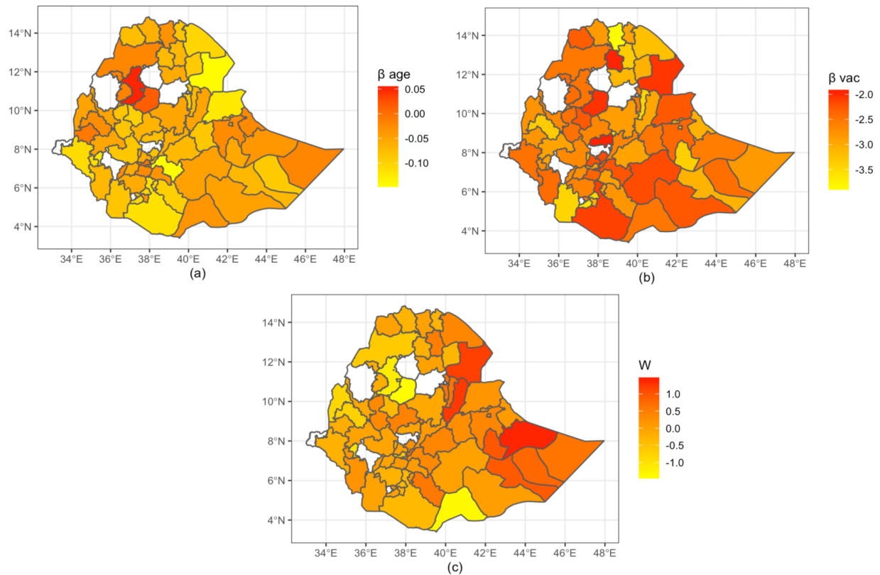
Figure 4: (a) Coefficients of age (b) Coefficients of vaccination (c) Random effects in V-SLR model on map of Ethiopia.
