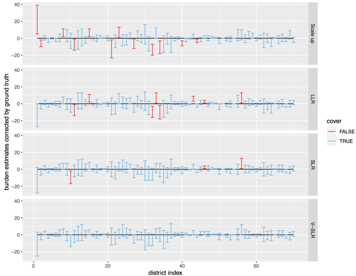
Figure 5: 95% confidence interval for burden estimates of scaling method, LLR, SLR and V-SLR model on district level.
