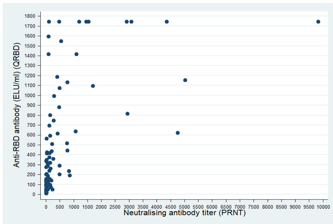
Figure 4: Scatter plot of Anti-RBD antibodies (ELU/ml) among participants with Neutralising antibody titre among them
