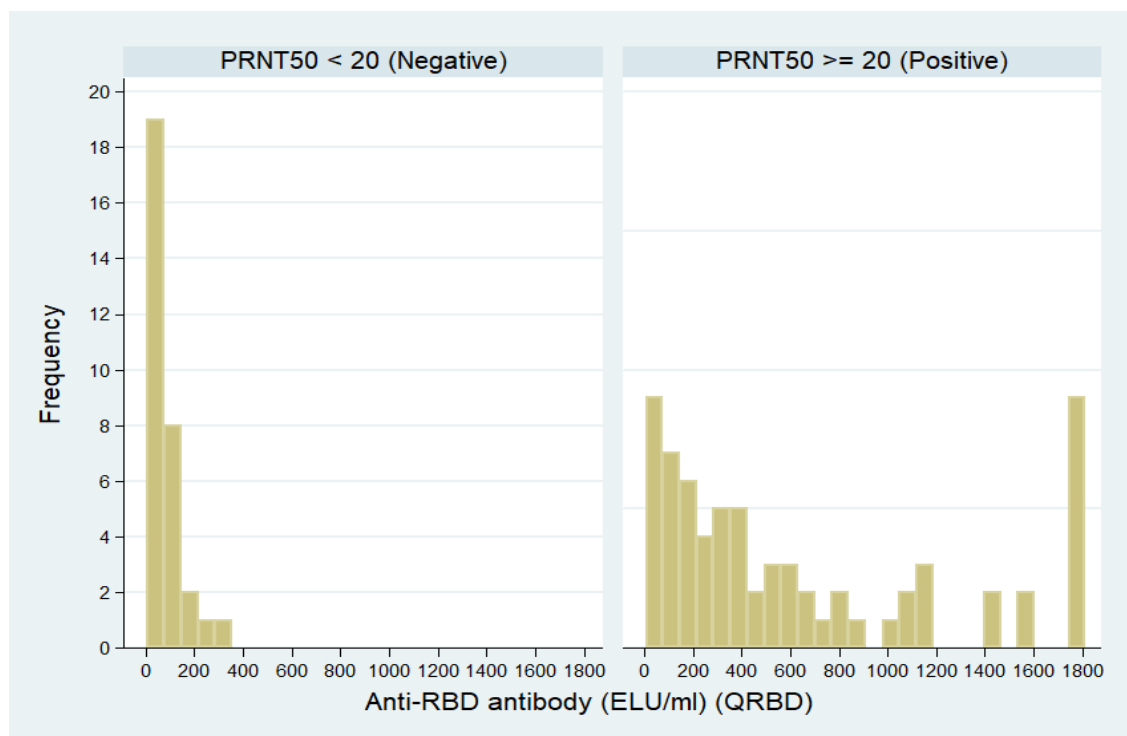
Figure 5: Histogram showing Anti-RBD antibodies (ELU/ml) among the participants with respect to PRNT_{50} < 20 and PRNT_{50} \geq 20 .
