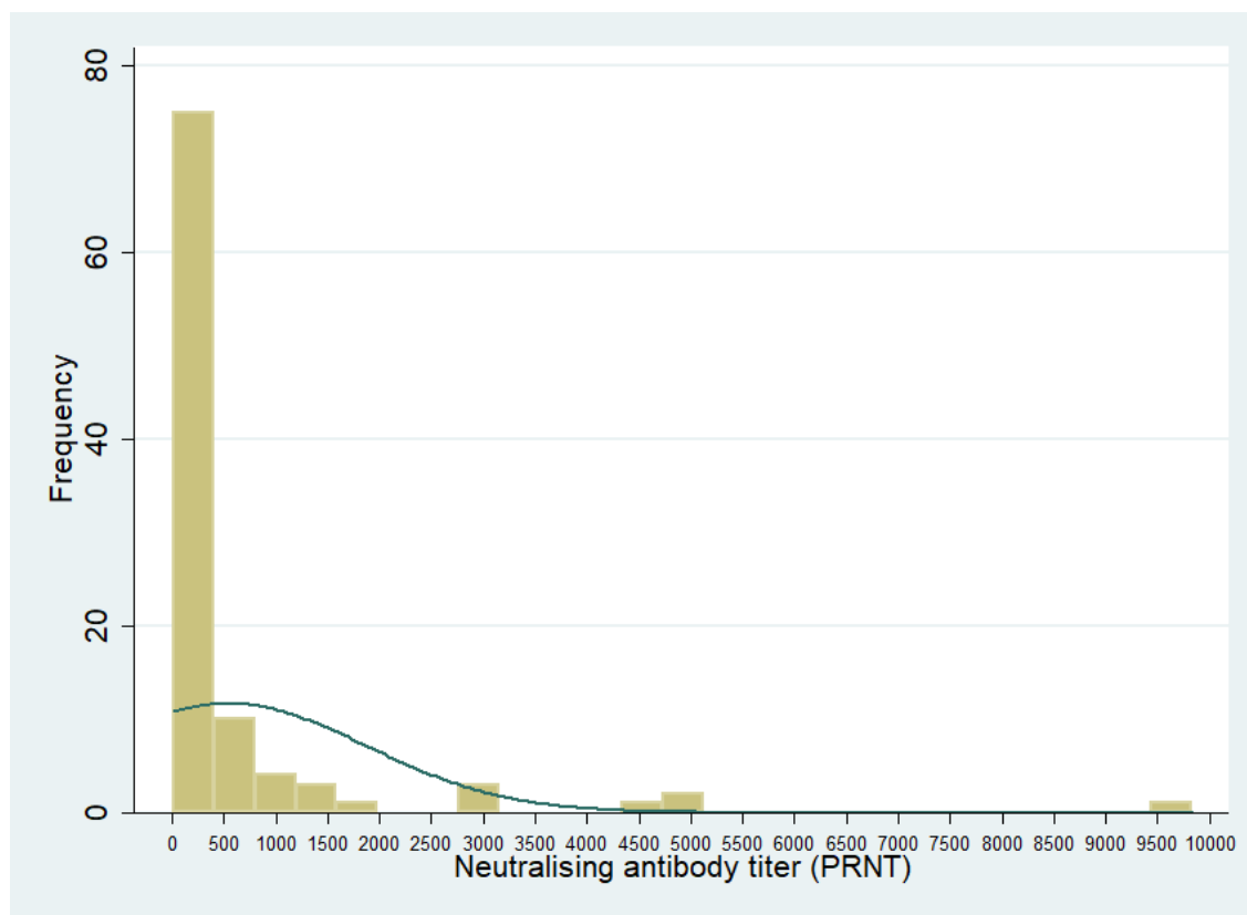
Figure 3: Distribution of Neutralising antibody titre among the participants
