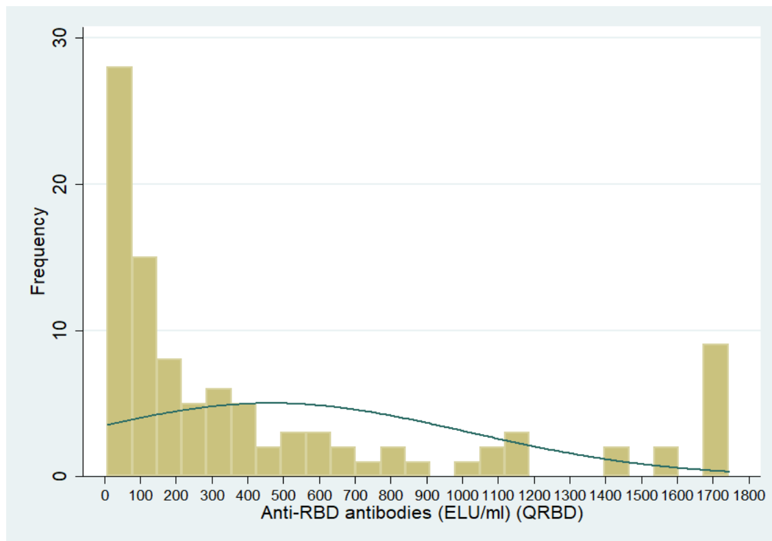
Figure 2: Distribution of Anti-RBD antibodies (ELU/ml) among study participants
