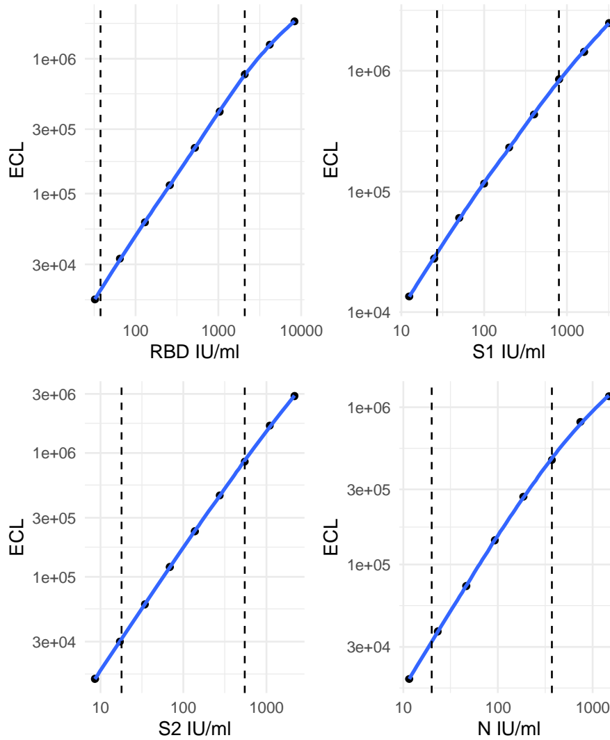
Figure 2. Standard curves for each component antigen in the CEPHR assay.
