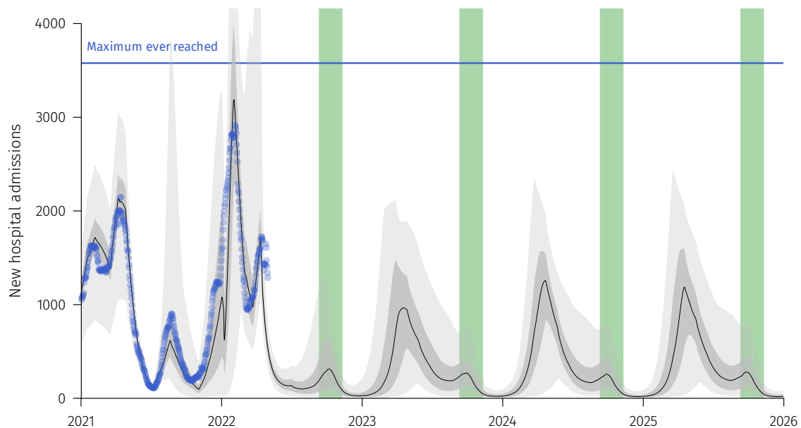
Figure S6: Detailed output of Scenario C (yearly vaccination of all the population) with a 20% reduction of the contact rate. See Figure S2 for additional details.
