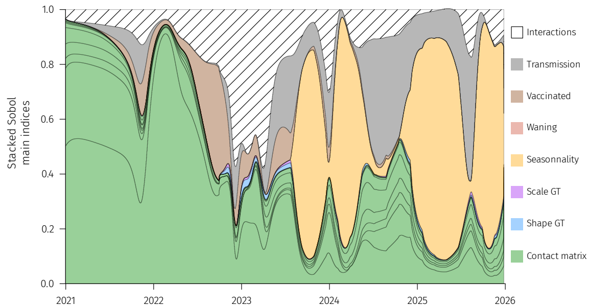
Figure S7: Global sensitivity analysis for Scenario A. The graphs shows the origin of the variance captured by each model parameter using Sobol indices (see Reyné et alii, 2022 for methodological details). A large part of the variations originates from the unknowns in the contact matrix between ages, as in Reyné et alii, 2022 . The magnitude of seasonality also matters for the long-term trends, as well as the transmission rate (i.e. the intensity of the NPIs).
