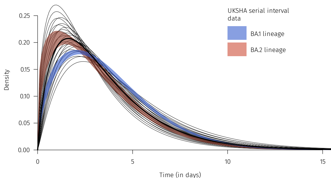
Figure S11: Omicron generation time. Shaded areas data originate from the UKSHA [2022] report. The lines correspond to a subset of the Gamma distributions used in the sensitivity analysis. The thicker line corresponds to the baseline Gamma distribution.
