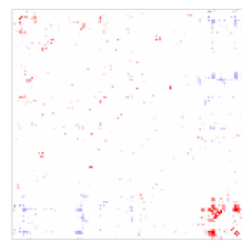
Differential functional connectivity in the cluster Pattern 2
