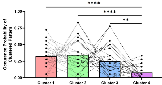
B Dynamic functional connectivity of IA patients in the second dataset
