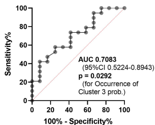
F The second dataset
