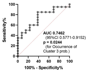
E The first dataset
