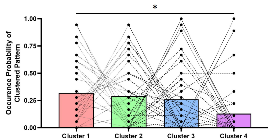
A Dynamic functional connectivity of IA patients in the first dataset
