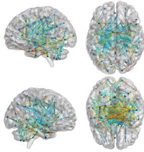
Fisher-transformed correlation coefficients -0.8 0.8
