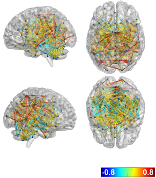
A Differential functional connectivity in cluster Pattern 3
