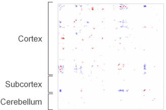
Differential functional connectivity in the cluster Pattern 1
