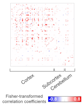
A Differential functional connectivity in cluster Pattern 3
