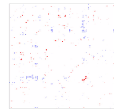
Differential functional connectivity in the cluster Pattern 4
