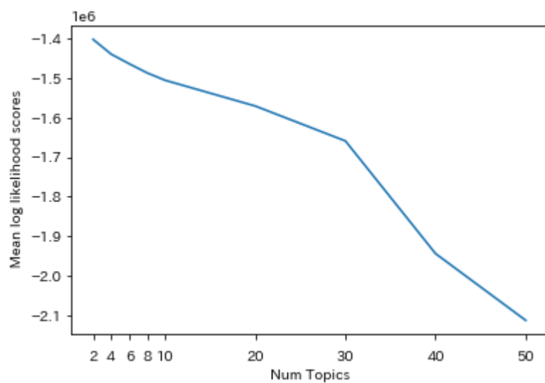
Fig. 1. Mean Log likelihood scores for different LDA topic numbers using five-fold cross validation.
