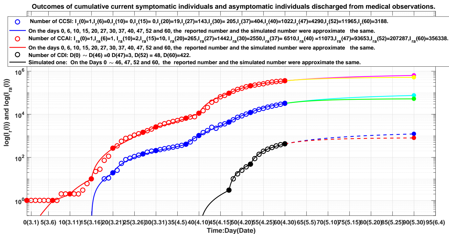
Figure 2 Blue circles: outcome of the number of the current cumulative recovered symptomatic individuals (CCSI), blue line: outcome of the corresponding simulations of equation (1). Red circles: outcome of the number of the current cumulative asymptomatic individuals (CCAI) discharged in medical medical observations, red line: outcome of the corresponding simulations of equation (1). Black circles: outcome of the number of the current cumulative died individuals (CCAI). Black line: outcome of the corresponding simulations of equation (1). The lines colored by cyan, magenta, green and yellow correspond to the virtual simulation results of equation (1). The dotted lines colored by blue and red corresponding to virtual simulation results for the cumulative died individuals. See Section Mainland Epidemic Virtual Simulations for details.
