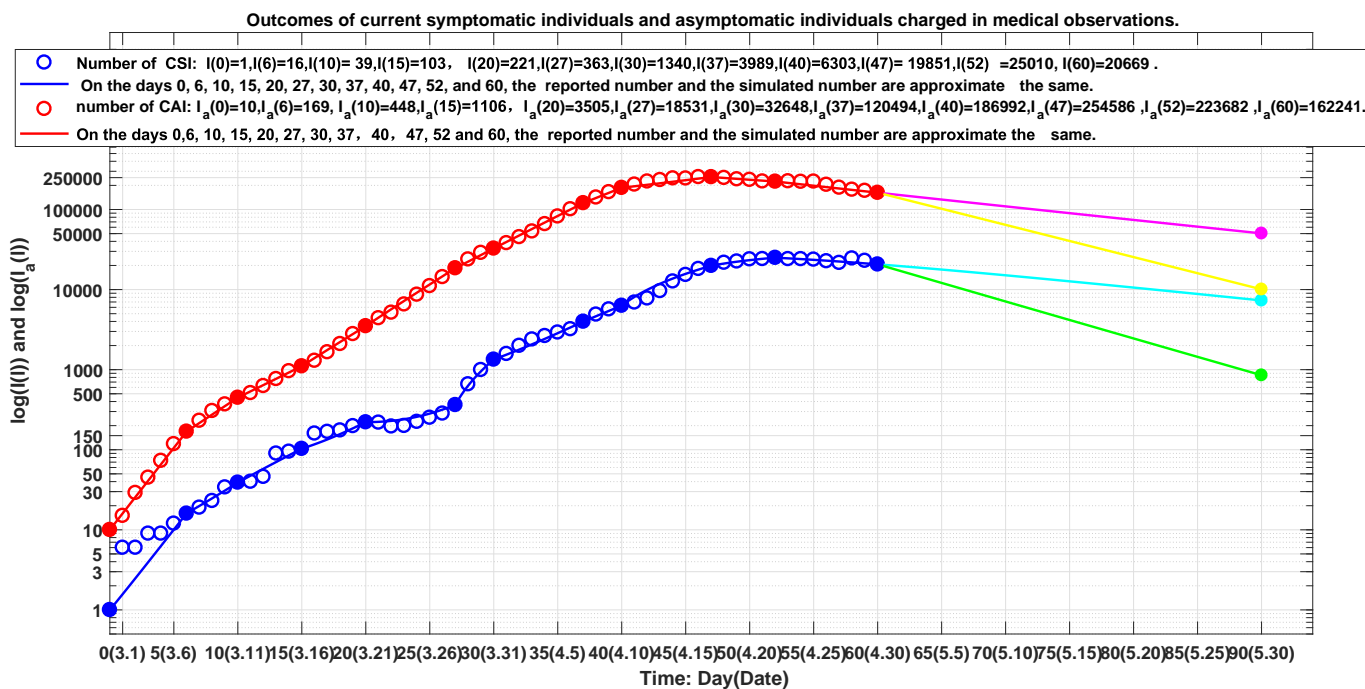
Figure 1 Blue circles: outcome of the number of the current symptomatic individuals (CSI), blue line: outcome of the corresponding simulation of equation (1). Red circles: outcome of the number of the current asymptomatic individuals (CAI) charged in medical observations, red line: outcome of the corresponding simulation of equation (1). The lines colored by cyan, magenta, green and yellow correspond the virtual simulation results of equation (1). See Section visual simulations for details.
