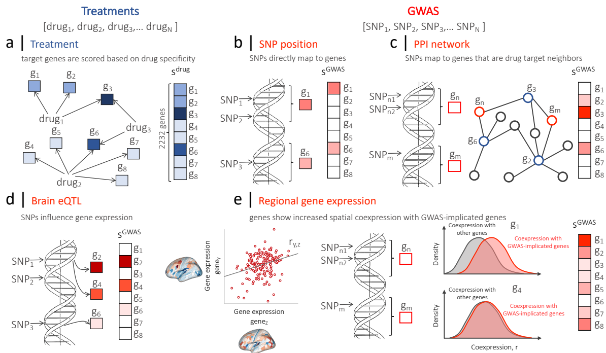
Figure 1. Evaluating the relationships between drug targets and GWAS by scoring genes based on: (i) their involvement in approved pharmaceutical treatments; and (ii) GWAS, for a given psychiatric disorder. (a) The analysis is based on a set of all clinically approved treatments. For each disorder, each of 2232 target genes derived from the DrugBank database 37 are assigned scores corresponding to their role as a target across drugs approved for use in treating that disorder. A gene is scored based on its specificity for each drug by assigning a value of w = 1/L , where L is the total number of targets for that drug. The total score for a gene is quantified as a sum of scores across drugs. For each disorder, the same set of 2232 genes is also scored based on their similarity to variants implicated in corresponding GWASs using four main methods for mapping SNPs to genes: (b) SNP position, where the SNPs are mapped to genes based on their position on the DNA and the gene score consequently proportional to the cumulative effect size of all SNPs mapped to that gene; (c) PPI network, where genes are scored based on the proportion of their direct neighbors that are implicated in GWAS (as mapped based on SNP position); (d) brain eQTL, where genes are scored based on the cumulative impact of GWAS-identified SNPs on influencing their expression; (e) regional gene-expression similarity calculated from the Allen Human Brain Atlas (AHBA). 38 First, for each pair of genes in the AHBA, the similarity of their spatial gene-expression profiles is quantified using a measure of gene-gene coexpression. Then, GWAS-implicated genes are identified based on SNP position and for each of 2232 target genes, coexpression value distributions are compared between GWAS-implicated and all other genes. As a result, a gene receives a high score if its coexpression with GWAS-implicated genes is, on average, higher than its coexpression with all other genes.
