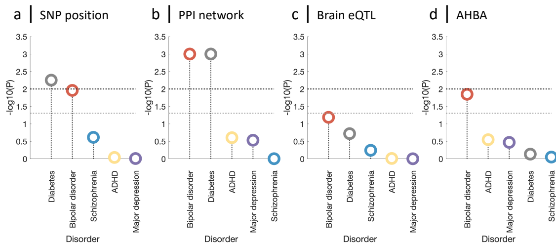
Figure 2. Bipolar disorder and diabetes demonstrate correspondence between treatment targets and genes implicated in GWAS data for each disorder. For a given disorder and mapping method, circles represent the significance of the association between the gene scores obtained from a set of drugs, s^{\text{drug}} , and GWAS data, s^{\text{GWAS}} , computed as a permutation test relative to a set of 5000 null scores generated from random drugs and plotted as -\log_{10}(p) [see details in eMethods 5 in Supplement 1]. Subplots correspond to the four GWAS mapping methods: (a) SNP position, (b) PPI network, (c) Brain eQTL, (d) Gene-expression similarity (cf. Fig. 1 b-e). Higher -\log_{10}(p) values indicate a stronger correspondence between GWAS and drug targets for a given disorder than expected from random treatments. Circles are colored by the disorder they represent (as labeled). Horizontal lines represent p-value thresholds: dark gray line – p = 0.01 (significant at \alpha = 0.05 after Bonferroni correction for five disorders); light gray line – p = 0.05 .
