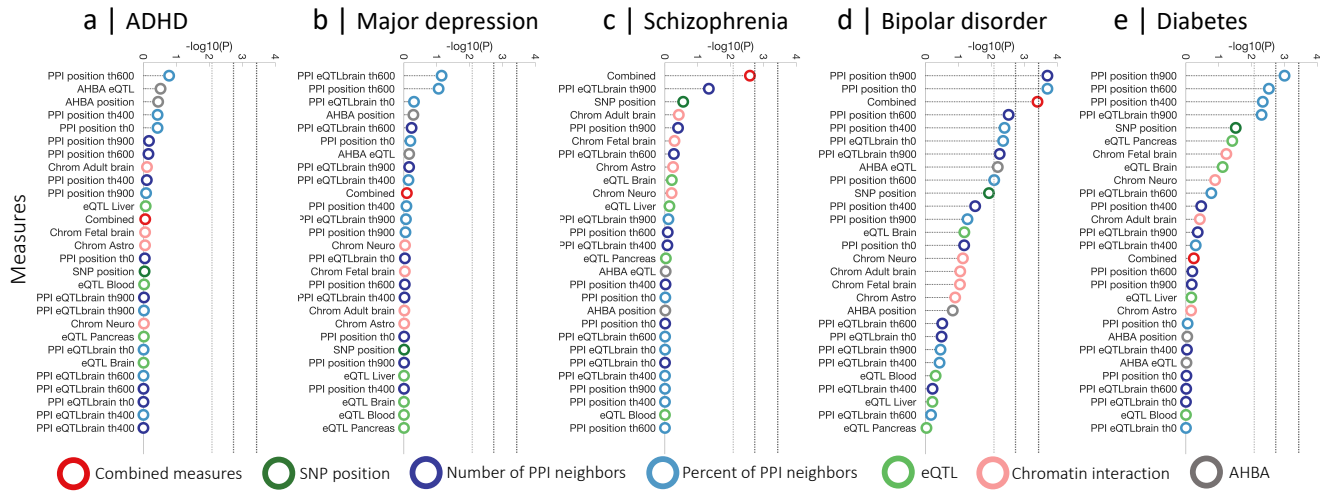
Fig. 3. PPI-based mapping methods show the strongest correspondence between treatment targets and genes implicated in a GWAS for bipolar disorder and diabetes. Circles represent the significance of the association between the treatment-based score, s^{\text{drug}} , and GWAS-based score, s^{\text{GWAS}} , for a selected disorder. The significance is quantified using a permutation-based p -value comparing the empirical GWAS-treatment matching score \rho to a set of 5000 matching scores generated using a selection of random drugs [see Online methods ]. The position of the circle corresponds to -\log_{10}(p) where higher values indicate more significant association. Subplots correspond to different disorders: (a) ADHD, (b) major depression, (c) schizophrenia, (d) bipolar disorder and (e) diabetes. Colors indicate different types of mapping methods: SNP position (dark green); spatial transcriptomic similarity (gray); chromatin interaction, Hi-c (pink); PPI network quantified as the proportion of neighbors (light blue); PPI network quantified as the total number of neighbors (dark blue); and eQTL (light green); linear combination of all measures (red). Horizontal lines represent the degree of statistical significance: light gray line -p^{\text{perm}} = 8.3 \times 10^{-3} (Bonferroni correction for six types of measures, this threshold provides guidance for the expected significance level considering that groups of measures derived from the same type of mapping method show a degree of similarity); dark gray line -p^{\text{perm}} = 1.9 \times 10^{-3} (Bonferroni correction for 27 measures); black line -p^{\text{perm}} = 3.7 \times 10^{-4} (Bonferroni correction for 27 measures and 5 disorders, this threshold provides guidance for a highly conservative correction assuming independence among all mapping methods and disorders). Permutation-based approach estimates a p -value with a minimum resolution of 2 \times 10^{-4} (corresponding to 1/5000). If the estimated p -value is lower, we conservatively place it at 2 \times 10^{-4} .
