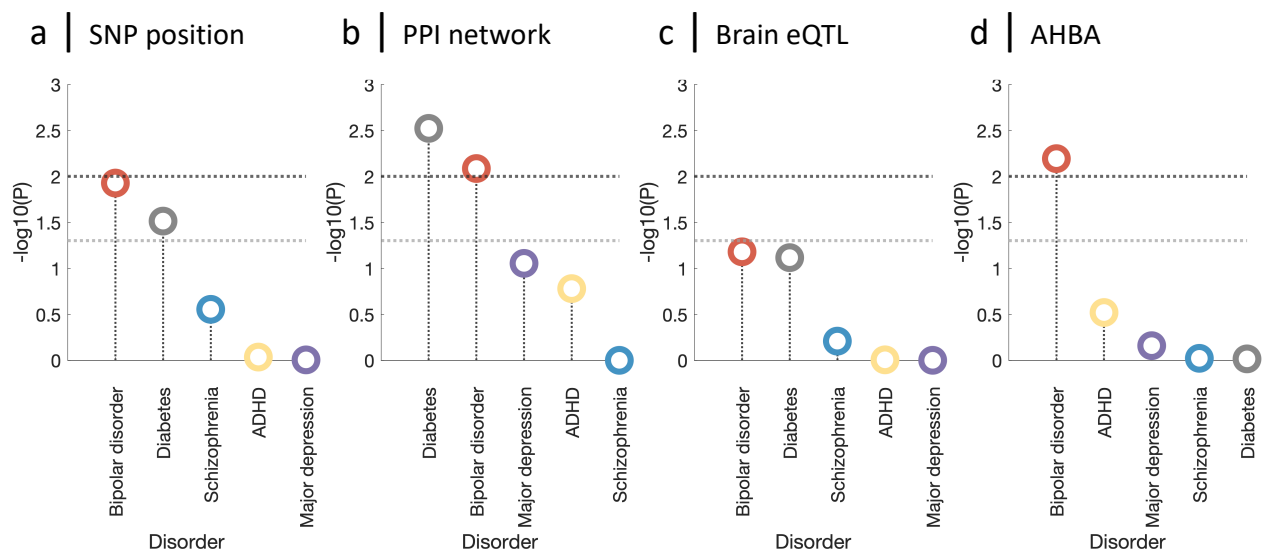
Fig. 2. Bipolar disorder and diabetes demonstrate correspondence between treatment targets and genes implicated in GWAS data for each disorder. For a given disorder and mapping method, circles represent the significance of the association between the gene scores obtained from a set of drugs, s_i^{\text{drug}} , and GWAS data, s_i^{\text{GWAS}} , computed as a permutation test relative to random drugs and plotted as -\log_{10}(p) [see Online methods ]. Subplots correspond to the four GWAS mapping methods: (a) SNP position, (b) PPI network, (c) Brain eQTL, (d) Gene-expression similarity (cf. Figs 1b–e). Higher -\log_{10}(p) values indicate a stronger correspondence between GWAS and drug targets for a given disorder than expected from random treatments. Circles are colored by the disorder they represent (as labeled). Horizontal lines represent p -value thresholds: dark gray line -p = 0.01 (significant at \alpha = 0.05 after Bonferroni correction for five disorders); light gray line -p = 0.05 .
