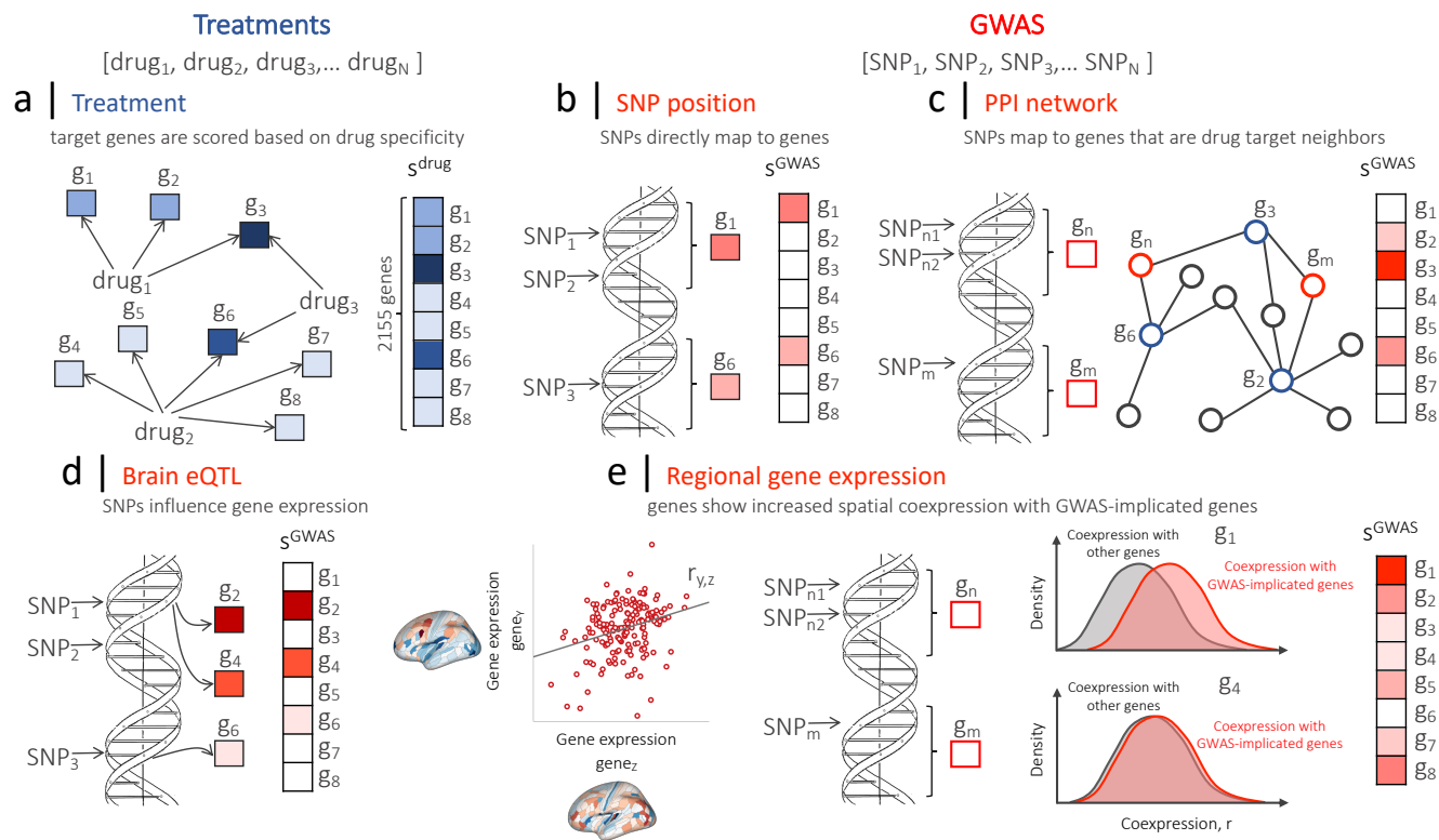
Fig. 1. We assess relationships between drug targets and GWAS by scoring genes based on: (i) their involvement in approved pharmaceutical treatments; and (ii) GWAS, for a given psychiatric disorder. (a) The analysis is based on a set of all clinically approved treatments. For each disorder, each of 2155 target genes derived from the DrugBank database (46) are assigned scores corresponding to their role as a target across drugs approved for use in treating that disorder. A gene is scored based on its specificity for each drug by assigning a value of w = 1/L , where L is the total number of targets for that drug. The total score for a gene is quantified as a sum of scores across drugs. For each disorder, the same set of 2155 genes is also scored based on their similarity to variants implicated in corresponding GWASs using four main methods for mapping SNPs to genes: (b) SNP position, where the SNPs are mapped to genes based on their position on the DNA and the gene score consequently proportional to the cumulative effect size of all SNPs mapped to that gene; (c) PPI network, where genes are scored based on the proportion of their direct neighbors that are implicated in GWAS (as mapped based on SNP position); (d) brain eQTL, where genes are scored based on the cumulative impact of GWAS-identified SNPs on influencing their expression; (e) regional gene-expression similarity calculated from the Allen Human Brain Atlas (AHBA) (47). First, for each pair of genes in the AHBA, the similarity of their spatial gene-expression profiles is quantified using a measure of gene–gene coexpression. Then, GWAS-implicated genes are identified based on SNP position and for each of 2155 target genes, coexpression value distributions are compared between GWAS-implicated and all other genes. As a result, a gene receives a high score if its coexpression with GWAS-implicated genes is, on average, higher than its coexpression with all other genes.
