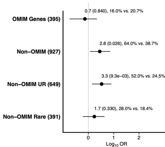
Figure 3: Children with viral respiratory failure harbor ultra-rare loss-of-function genetic risk factors
