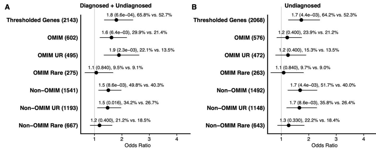
Figure 2: Gene-Set Enrichment Analysis Juxtaposing the Combined Cohort against the Unresolved Cohort
