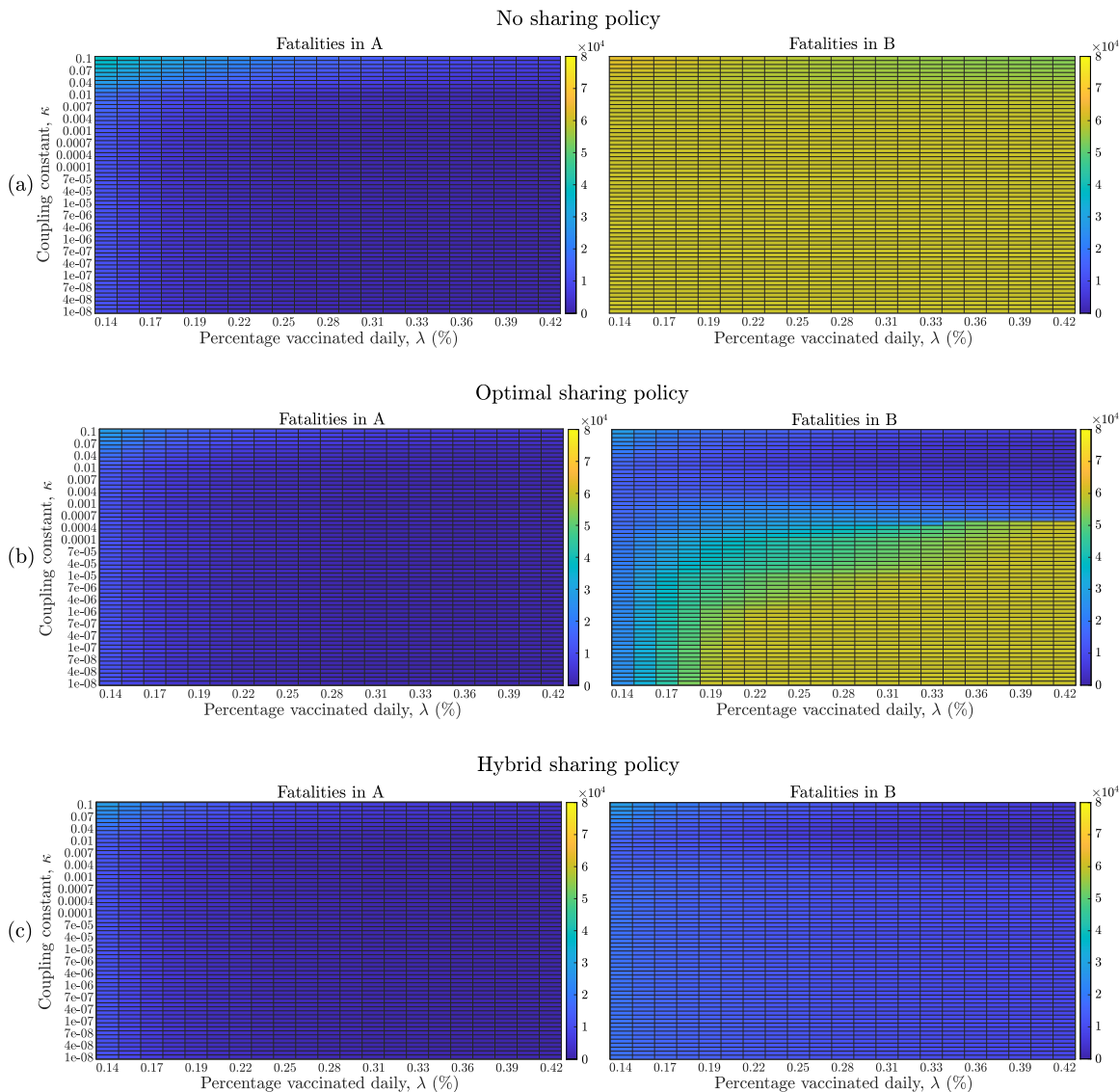
Figure S1: Fatalities in countries A and B when the (a) no-sharing policy, (b) optimal policy and (c) hybrid policy is implemented, over different coupling constants, \kappa \in [10^{-8}, 10^{-1}] and vaccination rates, \lambda (from 0.14% to 0.42% of the population daily). The optimal policy has the objective of minimizing fatalities in country A and the optimal sharing fraction is \mu^* . The hybrid policy is a near optimal policy with a sharing fraction of 1/3 when \mu^* \leq 1/3 and equal to the optimal sharing fraction otherwise. The optimal policy shows significant reduction in fatalities in B when vaccination rate is low and coupling constant is high, when compared to the no-sharing policy. The hybrid policy results in major reduction in fatalities in B for all vaccination rates and coupling constants, when compared to the no-sharing policy. There is a slight increase in fatalities in A for the hybrid policy when the coupling constant is very small and the vaccination rate is high.
