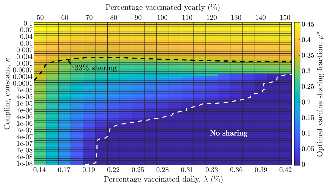
Figure 1: Dependence of the optimal fraction of vaccines ( \mu^* ) to be donated as a function of the vaccination rate, \lambda (x-axis) and the epidemic coupling coefficient, \kappa (y-axis). For very low values of \kappa and moderate to high vaccination rates, the optimal sharing fraction is 0. For all other values, the optimal vaccination donation fraction from country A to country B is positive, increasing with the epidemic coupling constant and the realized vaccination rate in country A. The black dashed line shows a level curve of \mu^* = 1/3 , while the white dashed line demarcates the region where \mu^* = 0 , that is, there is no vaccine sharing.
