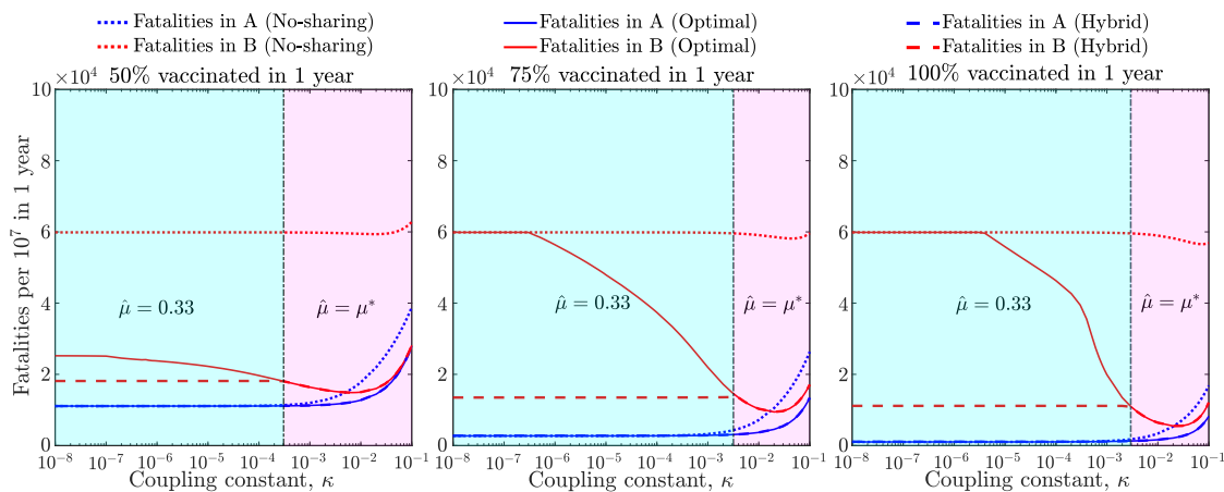
Figure 4: Fatalities per 10^7 over 1 year for the no-sharing, optimal and hybrid policies in countries A and B given different epidemic coupling constants ( \kappa \in [10^{-8}, 10^{-1}] ) and three vaccination rates (50%, 75% and 100% of the population vaccinated in 1 year). The hybrid policy maintains a vaccine sharing fraction of 0.33 to the left of the vertical black line, where the optimal vaccine sharing fraction is lower than 0.33 (shown here in cyan). To the right, the optimal vaccine sharing fraction is equal or greater than 0.33, so the hybrid vaccine sharing fraction is equal to the optimal in this region (shown here in magenta). The interpretation of the curves is same for each of the panels: blue denotes fatalities in A and red denotes fatalities in B. For each, the results are shown for no-sharing (dotted), optimal sharing (solid) and hybrid (dashed).
