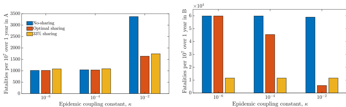
Figure 3: Fatality per 10^7 over 1 year in country A and B respectively for different sharing policies - no-sharing, optimal and 33% sharing. The daily vaccination rate is set as 0.28% of the total population. The two bar graphs list the total fatalities for all three policies (no-sharing, optimal and hybrid) shown in Fig. 2.
