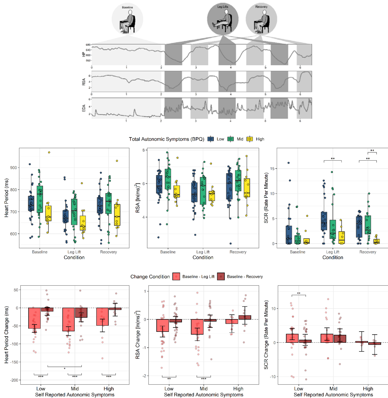
Figure 2. Autonomic activity changes during seated leg lifts as a function of level of autonomic symptoms self-reported on the Body Perception Questionnaire Short Form (BPQ-SF). Top row: Mean heart period (HP), respiratory sinus arrhythmia (RSA), and skin conductance reactivity (SCR) rate were measured during seated baseline, leg lifts, and recovery (legs on floor). Middle row: Raw data and boxplots with between-group significance tests from repeated measures models of absolute values at baseline, leg lifts, and recovery periods. For within-group contrasts see Supplemental Materials. HP and RSA models are adjusted for age and BMI. Bottom row: Linear mixed model predicted values and 95% confidence intervals for HP, RSA, and SCR rate change scores from baseline to leg lifts, and from baseline to recovery periods as a function of self-reported autonomic symptoms. Dotted horizontal lines designate no change.
