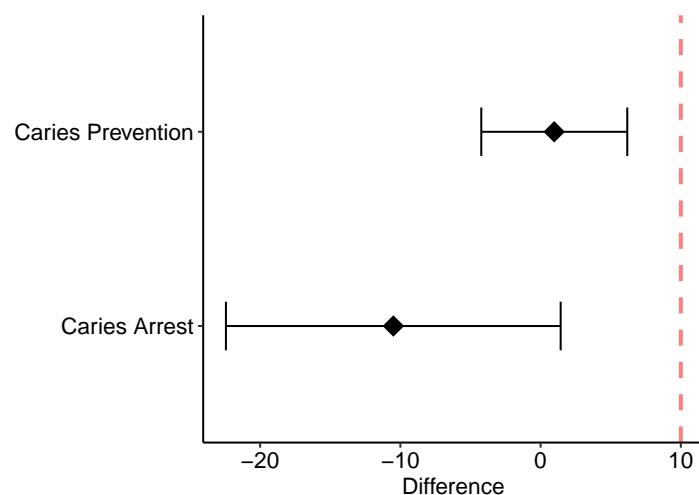
Figure 2: Non-inferiority plot for caries arrest and prevention at two years. The dashed red line denotes the non-inferiority limit.
