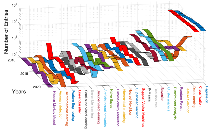
Fig. 6. Number of entries in PubMed per year and specific keyword related to Machine Learning Techniques. It should be noticed that entries related most techniques are fairly constant except for “Deep learning” which has increased constantly. It should be noticed that the vertical axis is logarithmic.
