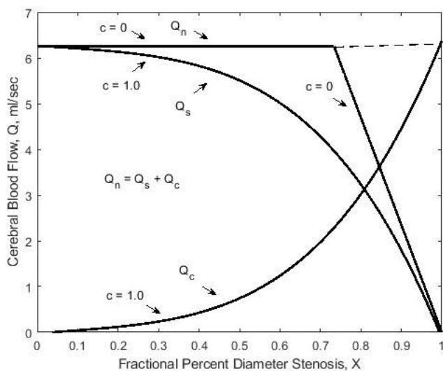
Figure 6. The two components of organ/tissue blood flow, stenotic artery, Q_s , and collateral Q_c , as a function of degree of stenosis when collateral magnitude C = 1.0 . When C = 0 , Q_c = 0 .
