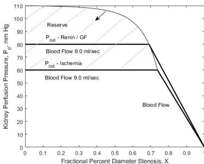
Figure 4. Numerical solution for kidney with two critical stenosis values, ischemia (74%) and glomerular filtration (71%). Actual blood flow has heavy lines.
