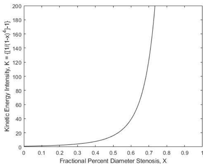
Figure 2. Arterial stenosis produced magnitude of dissipated energy, K , as function of fractional percent diameter stenosis, X .
