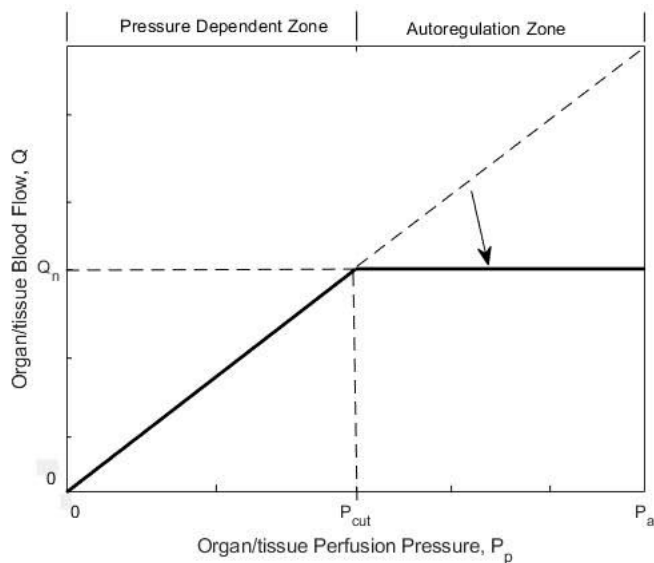
Figure 1. Schematic of Lassen cerebral blood flow autoregulation when organ/tissue perfusion pressure, P_p , is greater than pressure threshold, P_{cut} . Normal blood flow is Q_n .
