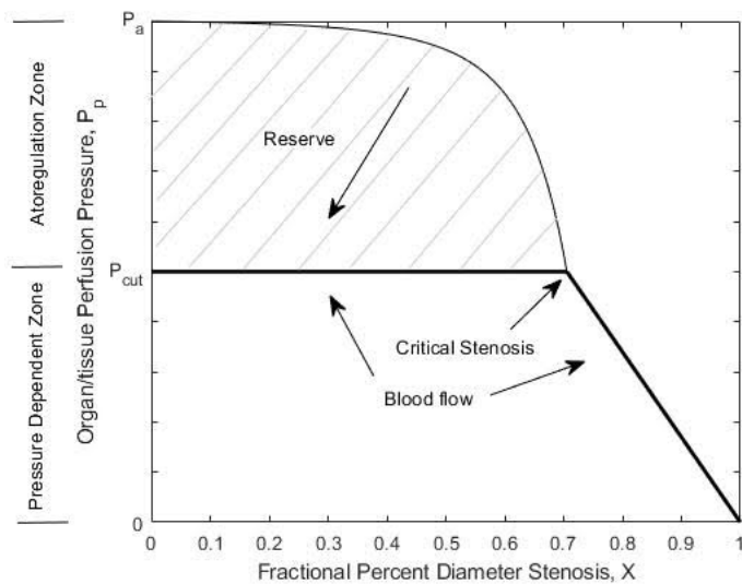
Figure 3. Energy solution for organ/tissue perfusion pressure and blood flow versus fractional percent diameter stenosis, X , in the absence of collaterals. Stenosis is critical when P_p reaches P_{cut} . Actual blood flow has heavy lines.
