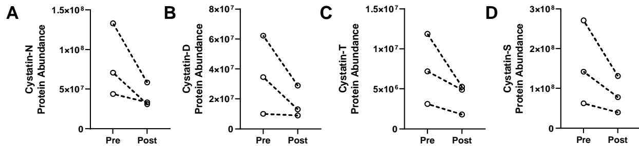
Figure 4. Human cystatin proteins with differential abundance. Protein abundances were plotted for the three subjects, with intraindividual pre- and post-octreotide values separated by a dotted line. Cystatin proteins which were significantly lower after octreotide treatment included (A) cystatin-SN (CYTN_HUMAN), (B) cystatin-D (CYTD_HUMAN), (C) cystatin-SA (CYTT_HUMAN) and (D) cystatin-S (CYTS_HUMAN). Data were plotted in GraphPad Prism.
