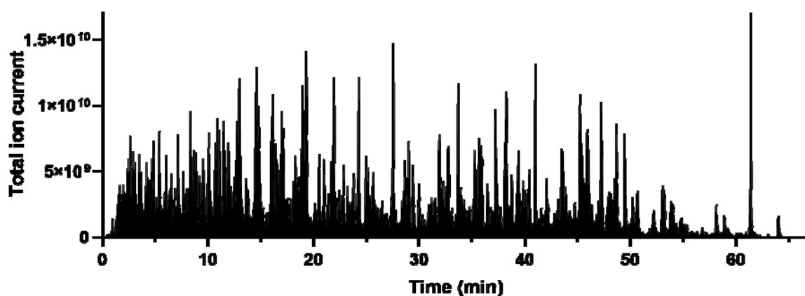
Figure 1. Representative chromatogram of tryptic digest of saliva. A tryptic digest ( \sim 40 \mu\text{g} ) was analyzed using microflow-LC-MS/MS and visualized as total ion current.
