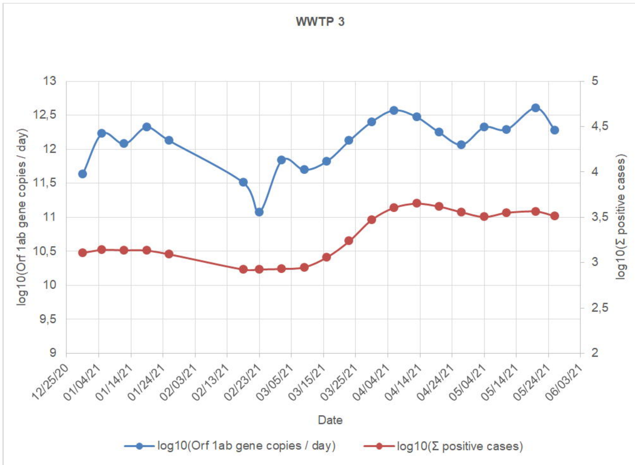
Figure 14. Evolution of Orf 1ab/day gene copies and accumulated positive cases (WWTP3).
