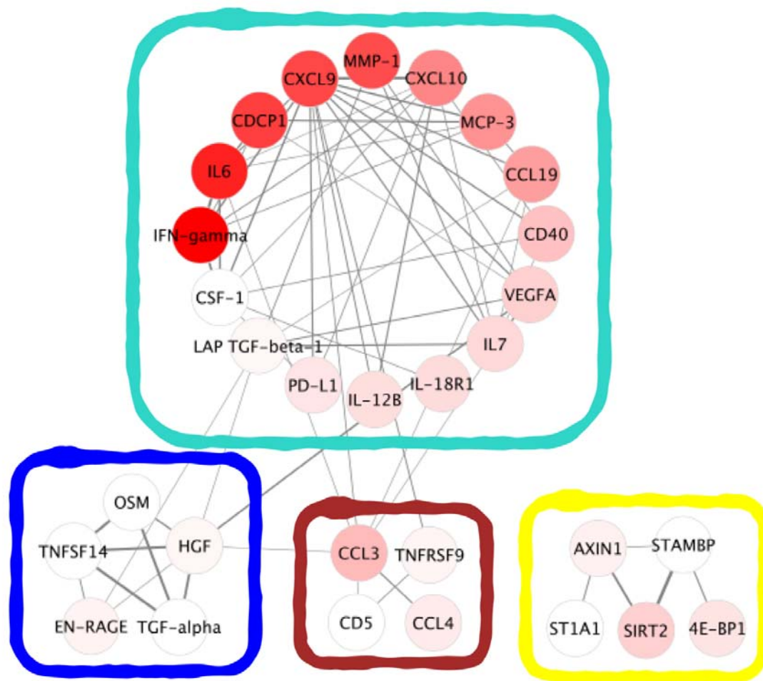
Figure 2. A visual representation of the protein co-expression network and the protein modules: The protein modules are surrounded by the colours turquoise, blue, brown or yellow. Nodes are coloured based on protein abundance (Fold Change) in comparison of active TB vs. control, with a darker red indicating a larger fold change. Links are depicted with thickness proportional to the correlation and only links representing Pearson's r > 0.6 are shown.
