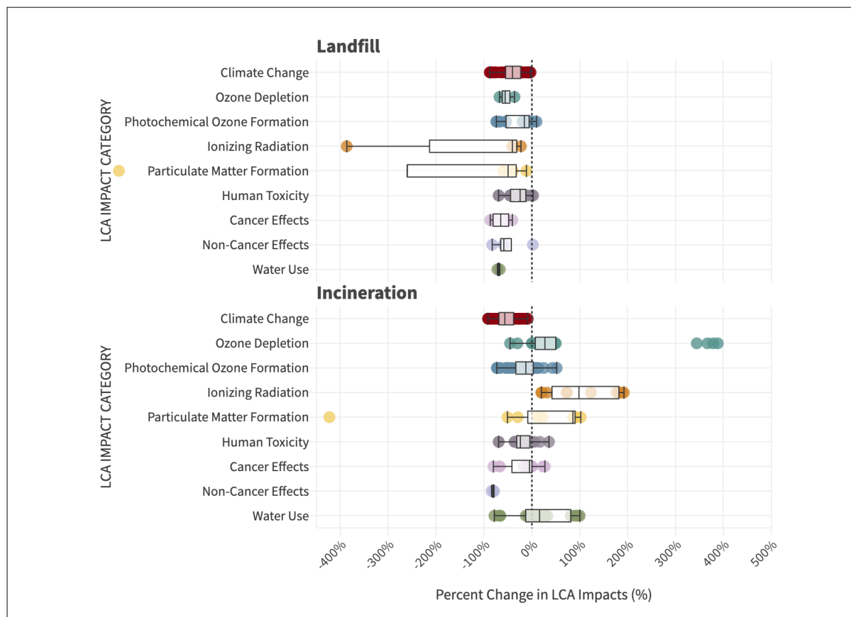
1341 1342 Fig. 7. Relative health-related impacts of 100% end-of-life plastic recycling. Percent 1343 change in health-related impacts, comparing 100% recycling to (A) 100% landfill 1344 and (B) 100% incineration. Values calculated for each comparison found within 1345 LCA studies are represented with dots and summarised using box plots of the 1346 median and interquartile range across data points for Climate Change, Ozone 1347 Depletion, Photochemical Ozone Formation, Ionizing Radiation, Particulate 1348 Matter Formation, Human Toxicity, Cancer Effects, Non-Cancer Effects and 1349 Water Use. 1350
