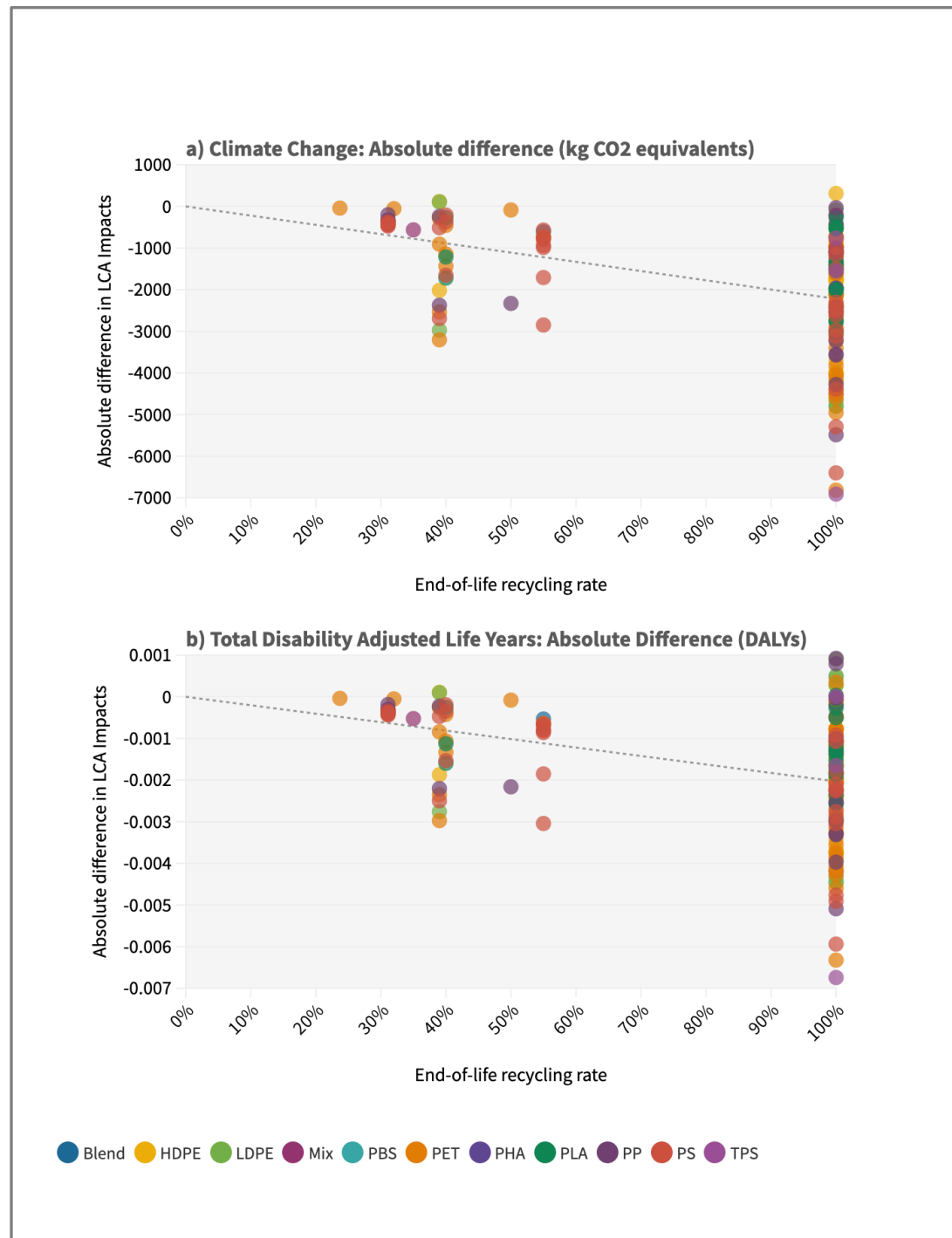
1351 1352 1353 1354 1355 1356 1357 1358 1359 Fig. 8. Meta-regression of the effects of increasing end-of-life recycling on Climate Change and Total DALYs. Scatter plot for mixed-effects linear regression with end-of-life recycling rate as the predictor variable and the response variables: (A) absolute difference in Climate Change impacts (kg CO 2 equivalents) relative to 0% recycling and (B) absolute difference in Total Disability-Adjusted Life Years (DALYs) based on multiple LCA health pathways, relative to 0% recycling. The key shows the colour coding of comparison points by plastic material type: Compound plastics (Blend), High-density Polyethylene (HDPE), Low-density
