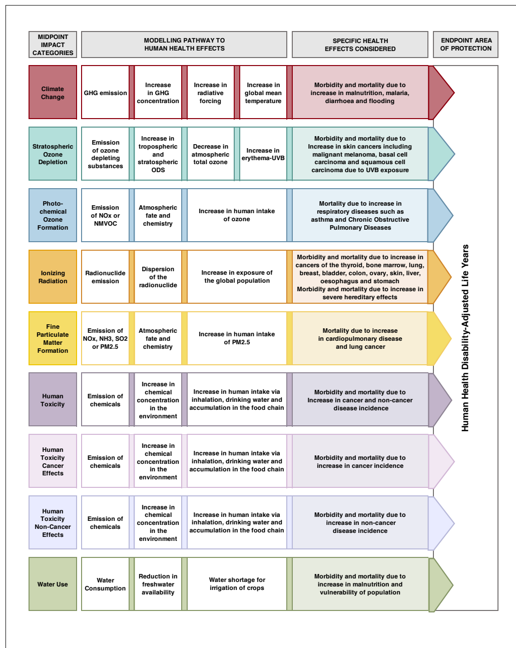
1281 1282 Fig. 1. Modelling human health effects in life cycle assessments. Life cycle assessment 1283 conceptual modelling process of health impact pathways from midpoint health- 1284 related categories to endpoint Human Health Disability-Adjusted Life Years 1285 (DALYs), according to ReCiPe 2016 life cycle impact assessment method. 1286 Authors' own: Adapted from ReCiPe 2016 v1.1 Report 1: Characterization. 2017 1287 (90). 1288
