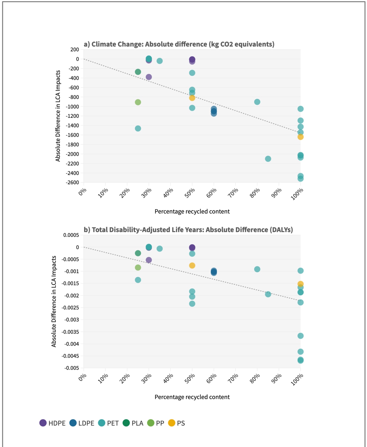
Fig. 6. Meta-regression of the effects of increasing recycled plastic content on Climate Change and Total DALYs. Scatter plot for mixed-effects linear regression with percentage recycled content as the predictor variable and the response variables: (A) absolute difference in Climate Change impacts (kg CO 2 equivalents) relative to virgin plastic packaging and (B) absolute difference in
