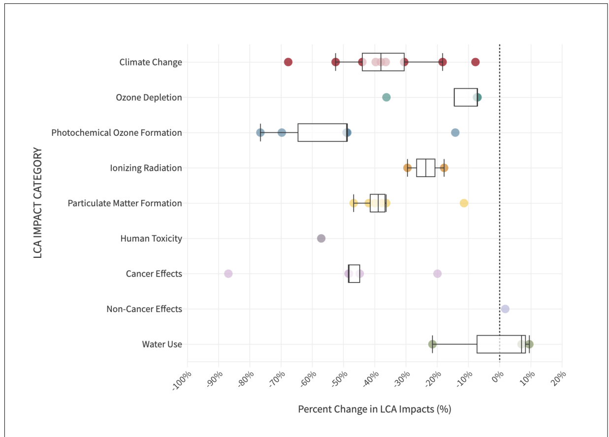
Fig. 5. Relative health-related impacts of 100% recycled plastic content. Percent change in health-related impacts, comparing 100% recycled plastic content products to virgin plastic products. Values calculated for each comparison found within LCA studies are represented with dots and summarised using box plots of the median and interquartile range across data points for Climate Change, Ozone Depletion, Photochemical Ozone Formation, Ionizing Radiation, Particulate Matter Formation, Human Toxicity, Cancer Effects, Non-Cancer Effects and Water Use.
