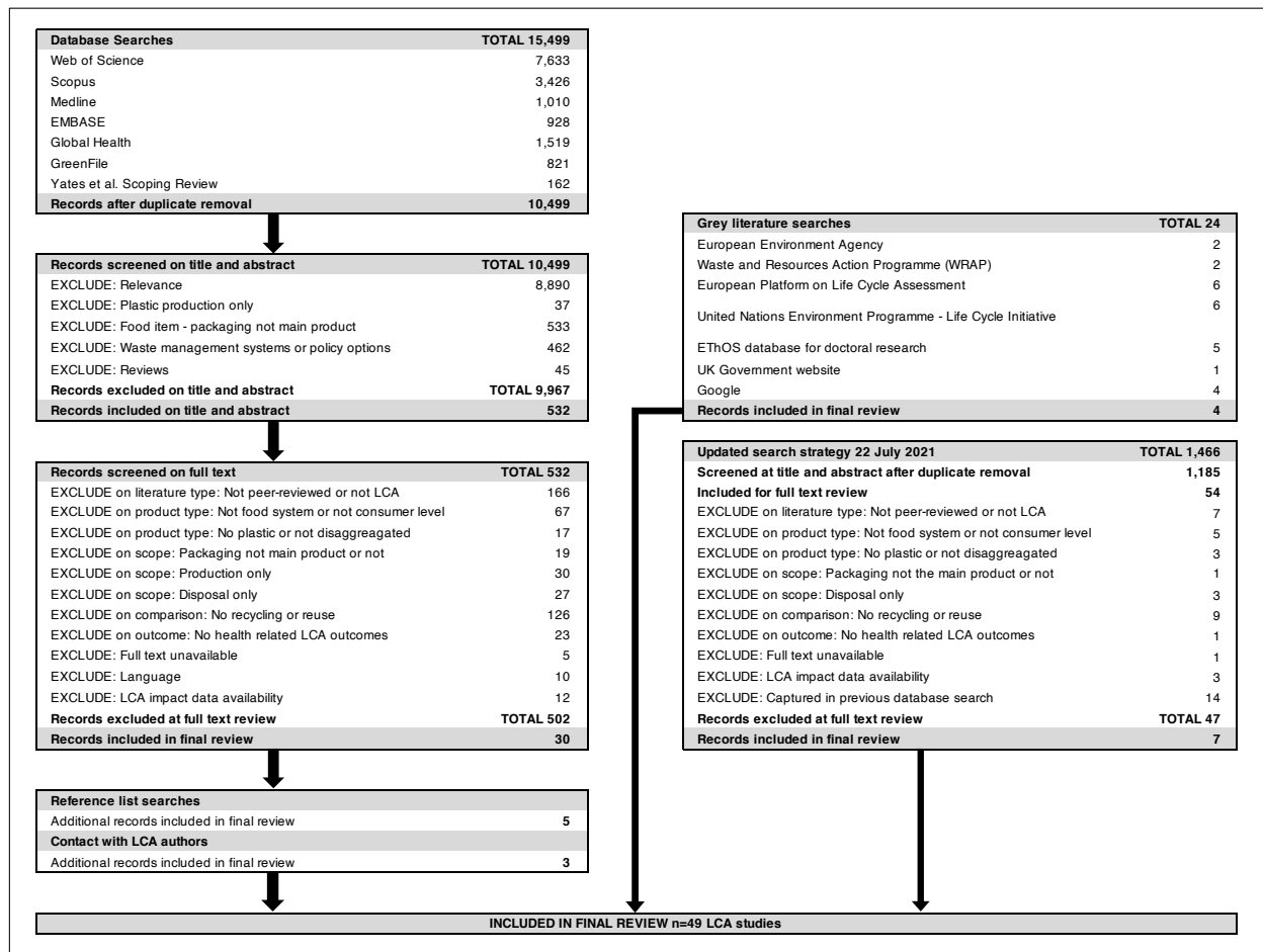
Fig. 3. PRISMA flow chart. Preferred Reporting Items for Systematic Reviews and Meta-Analyses (PRISMA) flow chart showing the study selection process for inclusion of life cycle assessments in the systematic review according to pre-defined eligibility criteria.
