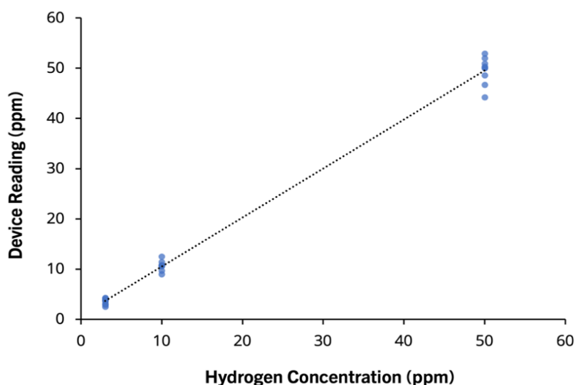
Figure 1. Linearity and repeatability curve for three AIRE devices tested at 3 ppm, 10 ppm and 50 ppm H 2 /air on three non-consecutive days.
