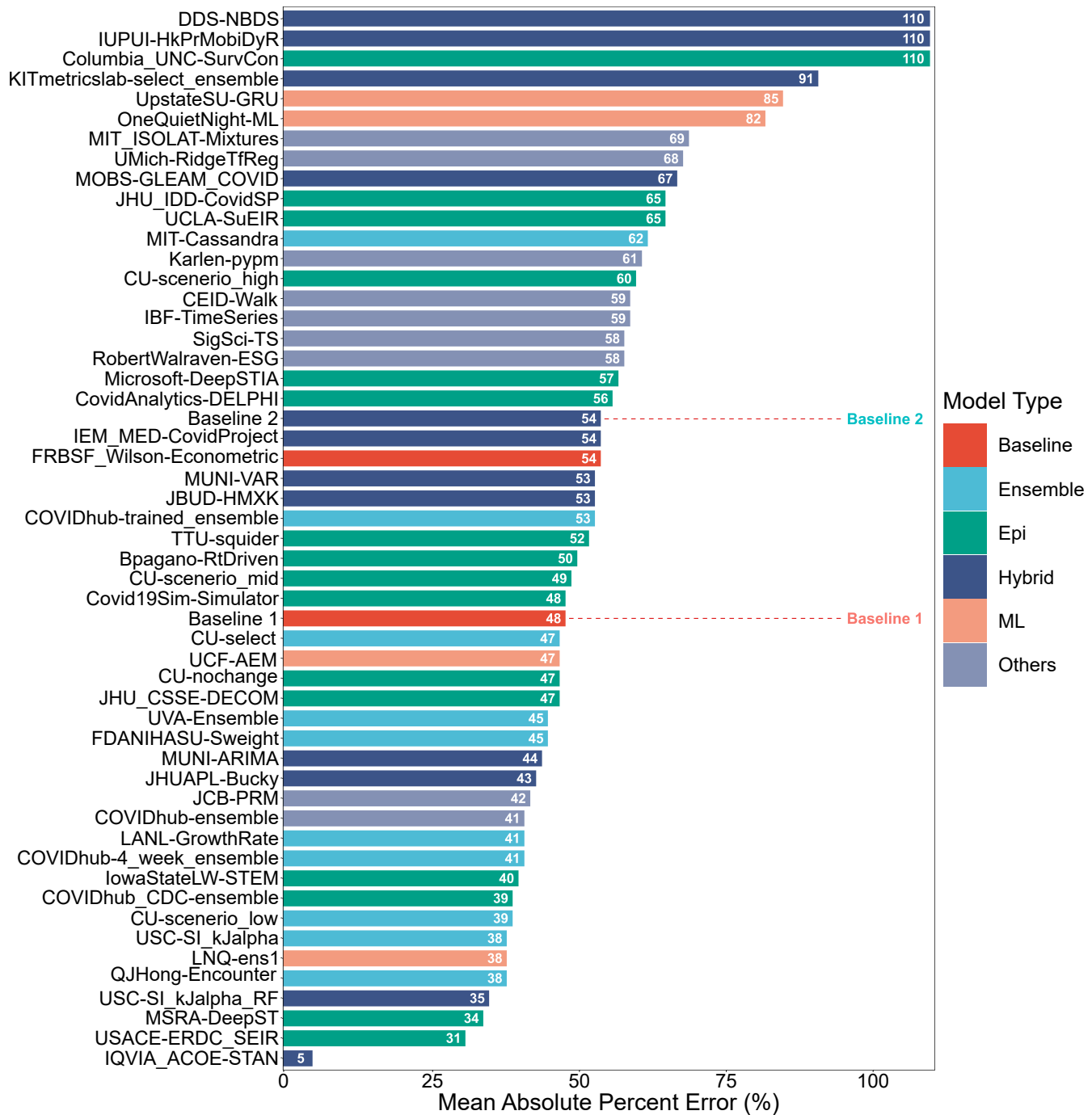
Figure 3. MAPE values of US-CDC case prediction models on the complete timeline, i.e., Wave-I to IV. The y-axis is sorted descending from lowest error to highest. The color scheme represents the model category.
