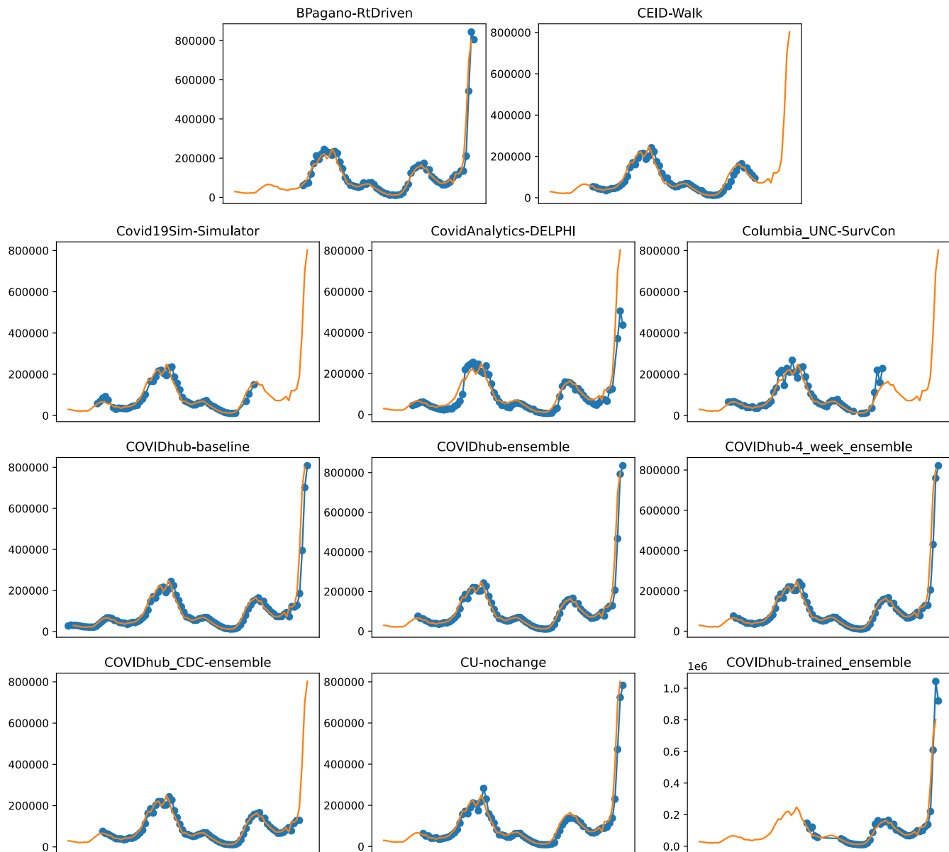
Figure 8. Plots depicting the peak predictions of US-CDC models- ‘BPagano-RtDriven’, ‘CEID-Walk’, ‘Covid19Sim-Simulator’, ‘CovidAnalytics-DELPHI’, ‘Columbia_UNC-SurvCon’, ‘COVIDhub-baseline’, ‘COVIDhub-ensemble’, ‘COVIDhub-4_week_ensemble’, ‘COVIDhub_CDC-ensemble’, ‘CU-nochange’, ‘COVIDhub-trained_ensemble’, over complete timeline
