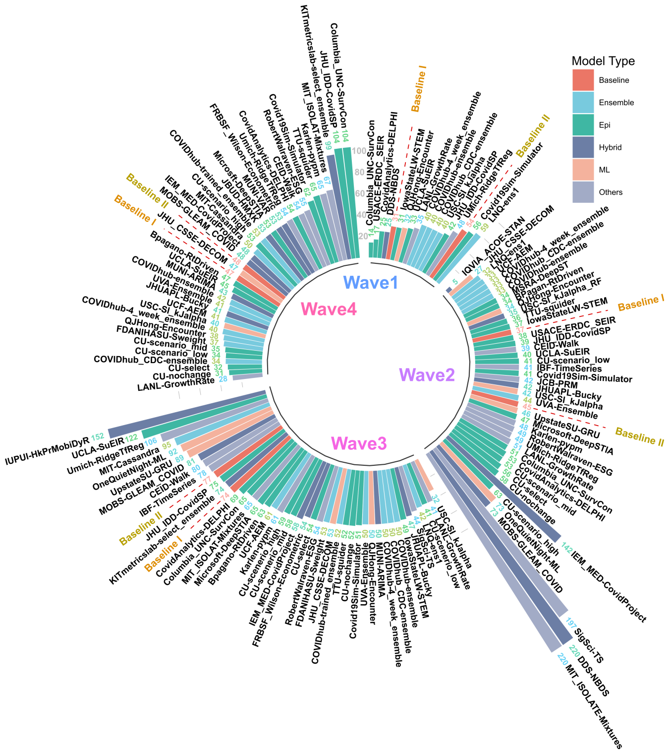
Figure 2. MAPE values of US CDC Case Prediction models in wave-I to IV. Models are sorted in descending order of MAPE. The color scheme represents the model category. Here “Baselines” are represented in red.
