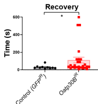
Fig. 4: a, UCSC browser exon view of Oatp30B in D. melanogaster (dm6 assembly) and SLCO5A1 in human (hg38 assembly). Pfam tracks show Oatp30B and SLCO5A1 have conserved MFS, OATP and Kazal domains. b, Startling reaction to trains of vibrations in flies with Oatp30B knock down. The UAS-Oatp30B IR (GD12775) transgenic or the control UAS-GFP IR were driven with nSyb-Gal4 and Ubi-Gal80ts . The w 1118 strain is a control for the genetic background in absence of transgenes. Mean +/- SEM ** p<0.01, One Way ANOVA, Tukey's post-hoc test. Units are the vibration events experienced 6 times for each fly. n=174-210. c, Increased seizure prevalence in flies with Oatp30B knock down. The UAS-Oatp30B IR (GD12775) transgenic or the control UAS-GFP IR were driven with nSyb-Gal4 and Ubi-Gal80ts . Percent +/- SE **** p<0.0001, Log-rank (Mantel-Cox) test, \chi^2 24.68 for 1 df, n=34-36. d, Increased post-seizure recovery time in flies with Oatp30B knock down. The UAS-Oatp30B IR (GD12775) transgenic or the control UAS-GFP IR were driven with nSyb-Gal4 and Ubi-Gal80ts . Mean +/- SEM * p<0.05, Mann Whitney non-parametric test, two tails, n=10-26. Only flies that displayed a seizure within 120 s as in Fig. 4b have been included in the analysis.
