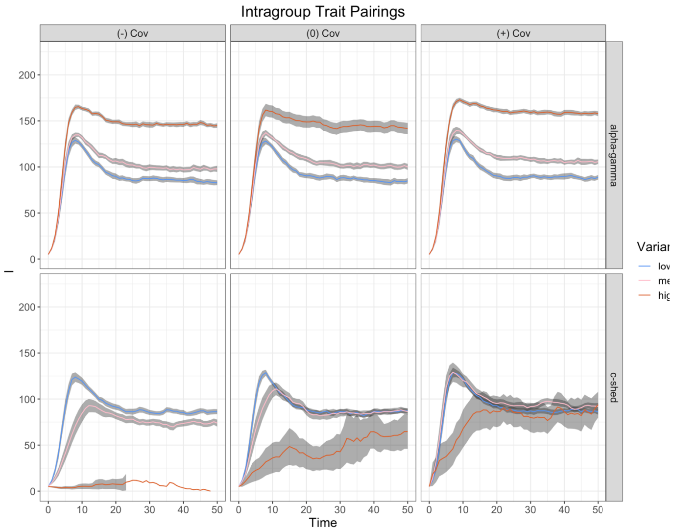
Figure 1. Dynamics of infected individuals over time for intragroup trait pairings at a moderate R_0 for all levels of variation and directions of covariation. For each simulation, the initial number of susceptible hosts is given by the expected equilibrium population size in the absence of infection, minus the initial number of infected hosts, which was always 5.
