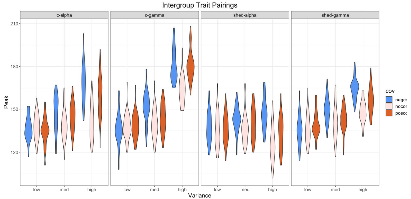
Figure 3. Distribution of peak epidemic sizes for intergroup trait pairings at all levels of variation and directions of covariation. Differences in violin width indicate the density of peak epidemic sizes at that value.
