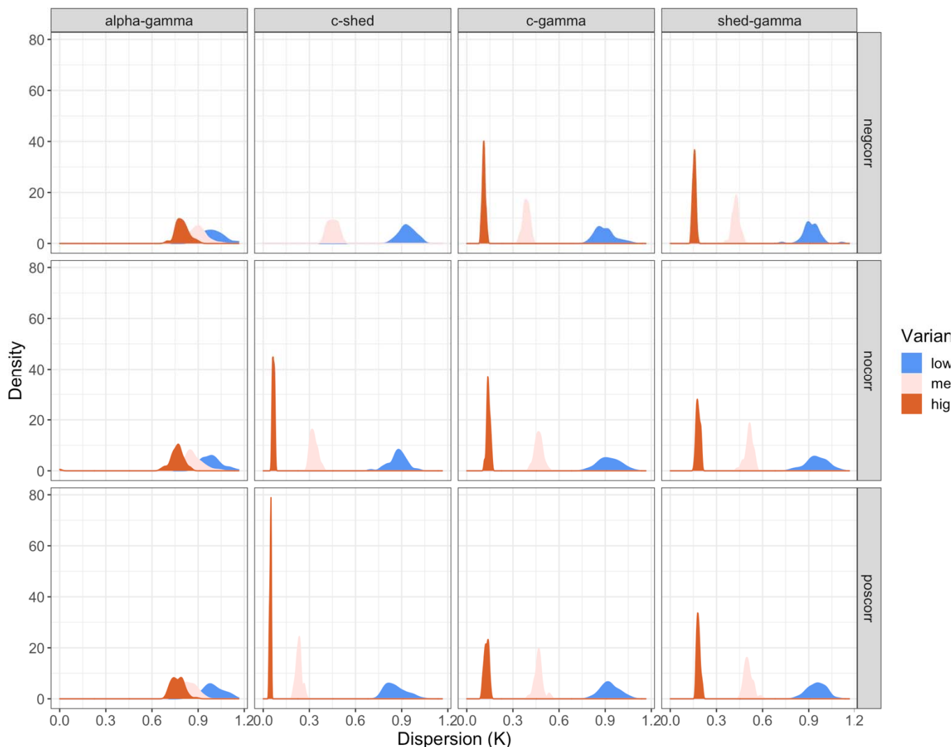
Figure 4. Distribution of dispersion (K) values for each trait pairing, level of variation and direction of covariation. Lower dispersion values indicate more super-spreading.
