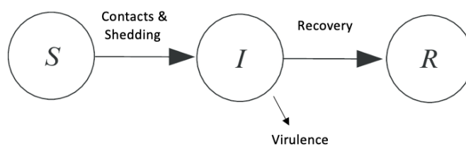
Figure 1. Flow diagram of SIR model. Contact and shedding determine movement from susceptible to infected, recovery determines movement from infected to recovered, and virulence determines infected individuals that do not recover. Births and deaths are not included in this diagram but are included in the SIR model used.
