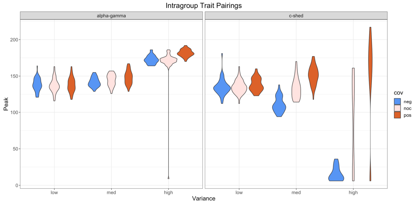
Figure 4. Distribution of peak epidemic sizes for intragroup trait pairings at all levels of variation and directions of covariation. Differences in violin width indicate the density of peak epidemic sizes at that value.
