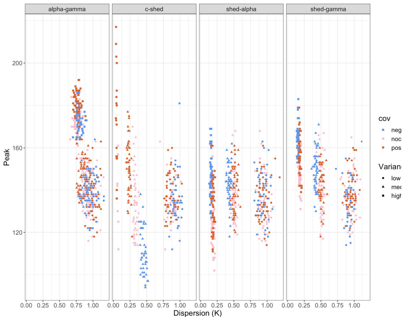
Figure 5. Relationship between dispersion ( K ) and peak epidemic size for all trait pairings, level of variance and direction of covariation.
