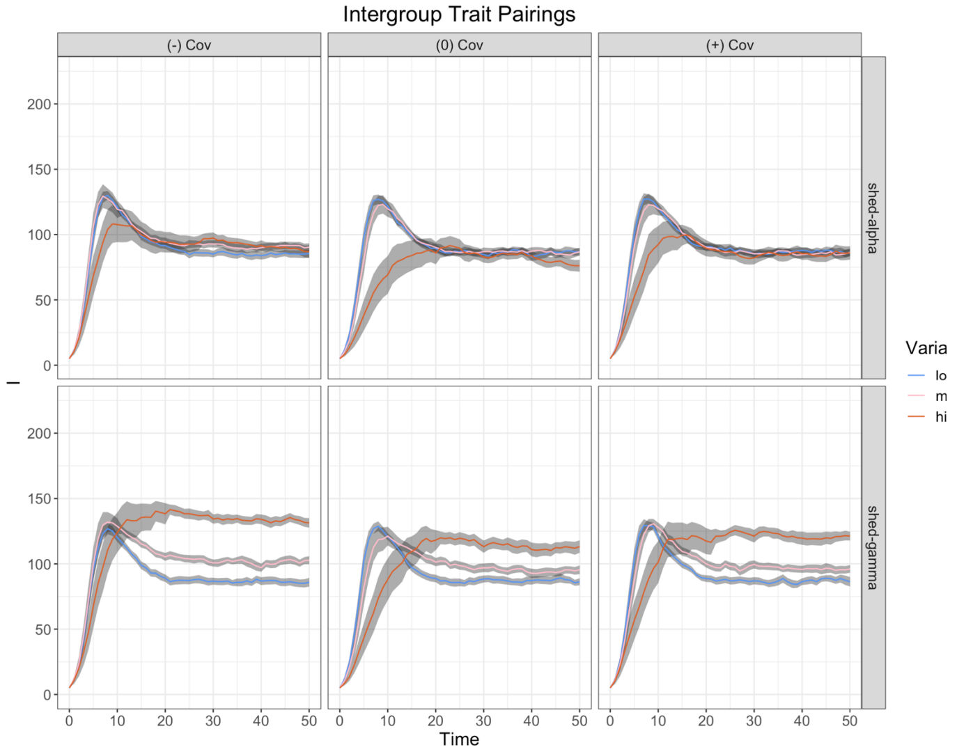
Figure 2. Dynamics of infected individuals over time for intergroup trait pairings at a moderate R_0 for all levels of variation and directions of covariation. Note that the trait pairings of contact with virulence (alpha) and recovery (gamma) are omitted but can be found in the appendix.
