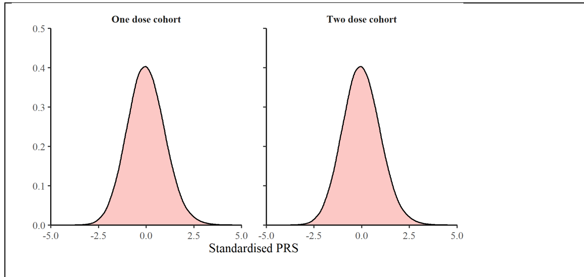
sFigure 1: Distribution of polygenic risk score for venous thromboembolism
