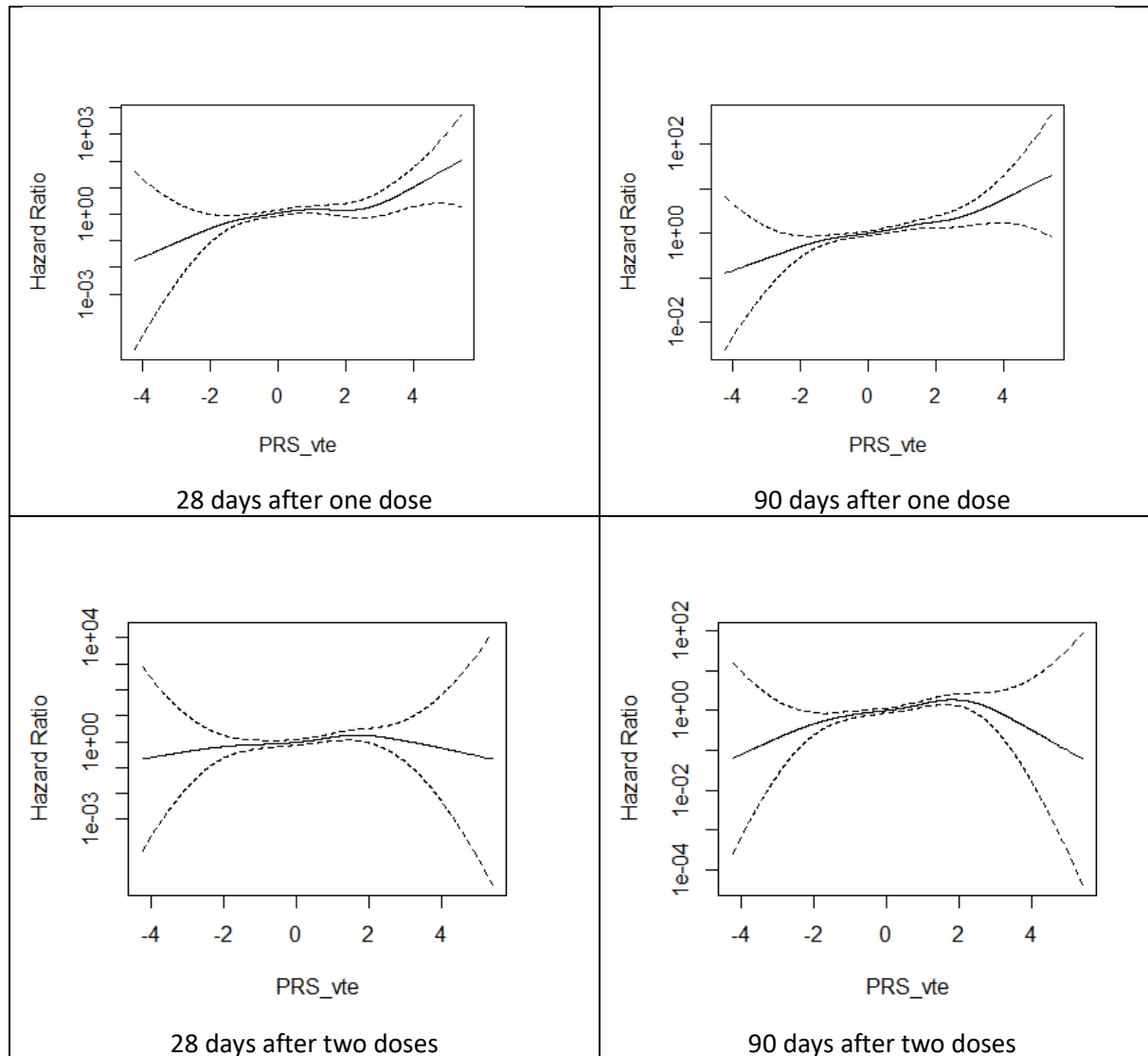
Figure 2: The relationship between the PRS value and the risk (hazard ratio) of VTE.
