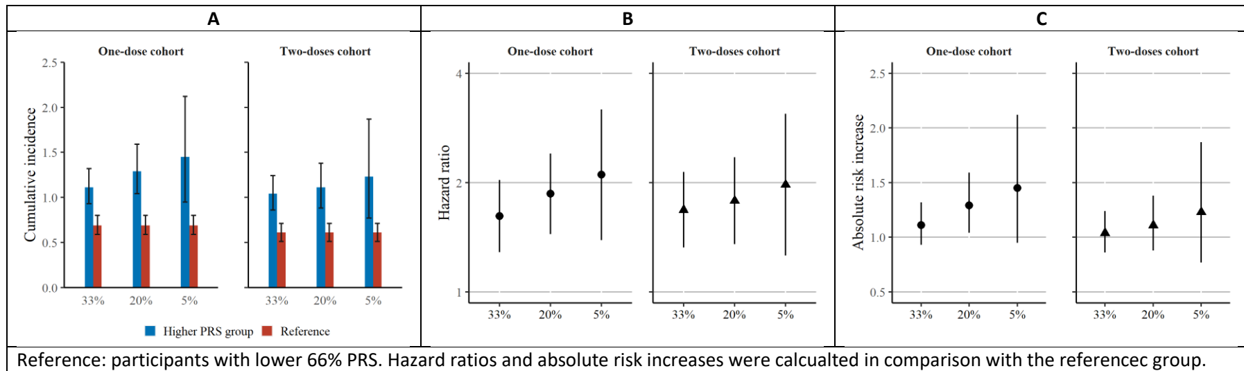
Figure 2: 90-day cumulative incidence (A), hazard ratios (B) and absolute risk increases (C) of three pre-defined high genetic risk groups vs the reference.
