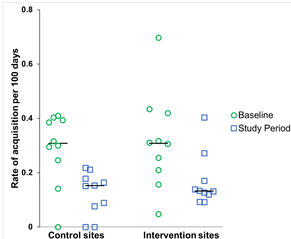
Figure 2: Rates of acquisition of 027-like C. difficile per 100 days in the baseline and study periods for the control and intervention ICUs.
