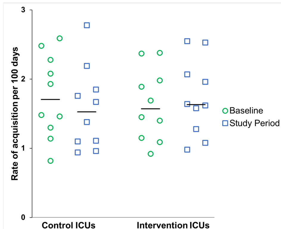
Figure 1. Rates of acquisition of toxigenic C. difficile per 100 days in the baseline and study periods for the control and intervention ICUs.
