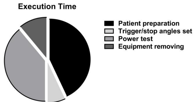
Figure 6: Execution time.
