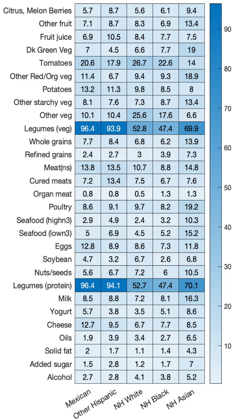
483 Figure 3. Heatmap illustrating probability of a given food item assuming a pattern at the global 484 level. Foods likely to assume a global pattern are darker in blue hue. Foods likely to assume a 485 localized pattern by the racial/ethnic subgroup are lighter in blue hue.
