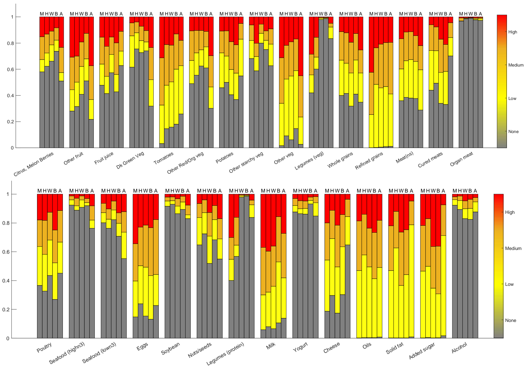
Figure 4. Pattern distributions for RPC-derived local profiles for each racial/ethnic subgroups. M=Mexican, H=Other Hispanic, W=Non-Hispanic White, B=Non-Hispanic Black, A=Non-Hispanic Asian.
