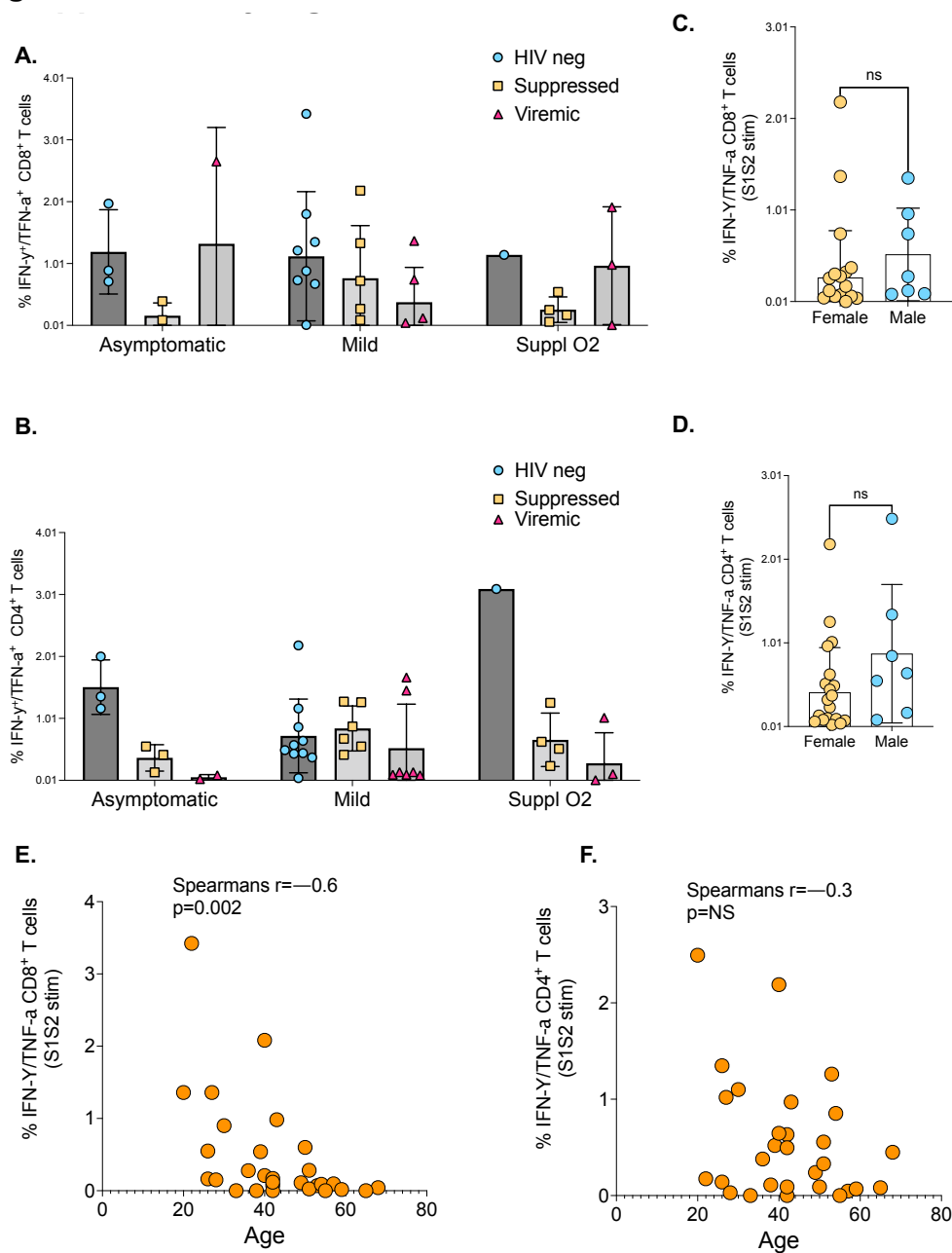
Figure S2. Assessment of the effect of COVID-19 disease severity on, (a) SARS-CoV-2 specific CD8 ^{+} , and (b) CD4 ^{+} T cell responses. Disease severity categorised as asymptomatic, mild, and on supplemental oxygen or death. (c,d) Analysis of SARS-CoV-2 responses based on gender. Correlation between age and SARS-CoV-2 specific, (e) CD8 ^{+} T and (f) CD4 ^{+} T cell responses. P-values calculated by Mann-Whitney U test and Pearson correlation test.
