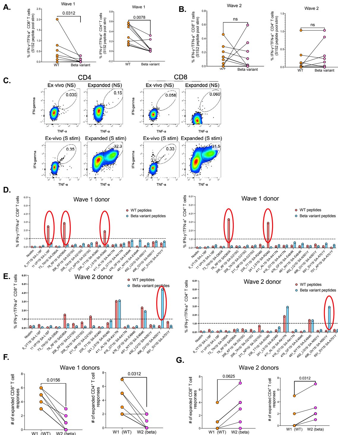
Figure 3: Poor cross-recognition of SARS-CoV-2-specific CD4 + and CD8 + T cell responses between wt and beta variants in wave 1 and wave 2 COVID-19 participants: Ex vivo assesment of T cell cross-recognition between the two
