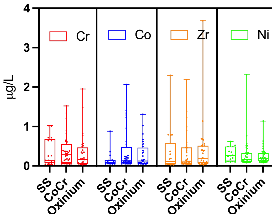
Figure 3. Boxplot of blood metal ion levels ( \mu\text{g/L} ) for Cr, Co, Zr and Ni, grouped on head material. Horizontal lines inside the box indicates median level. Whiskers represents min-max values (range).
