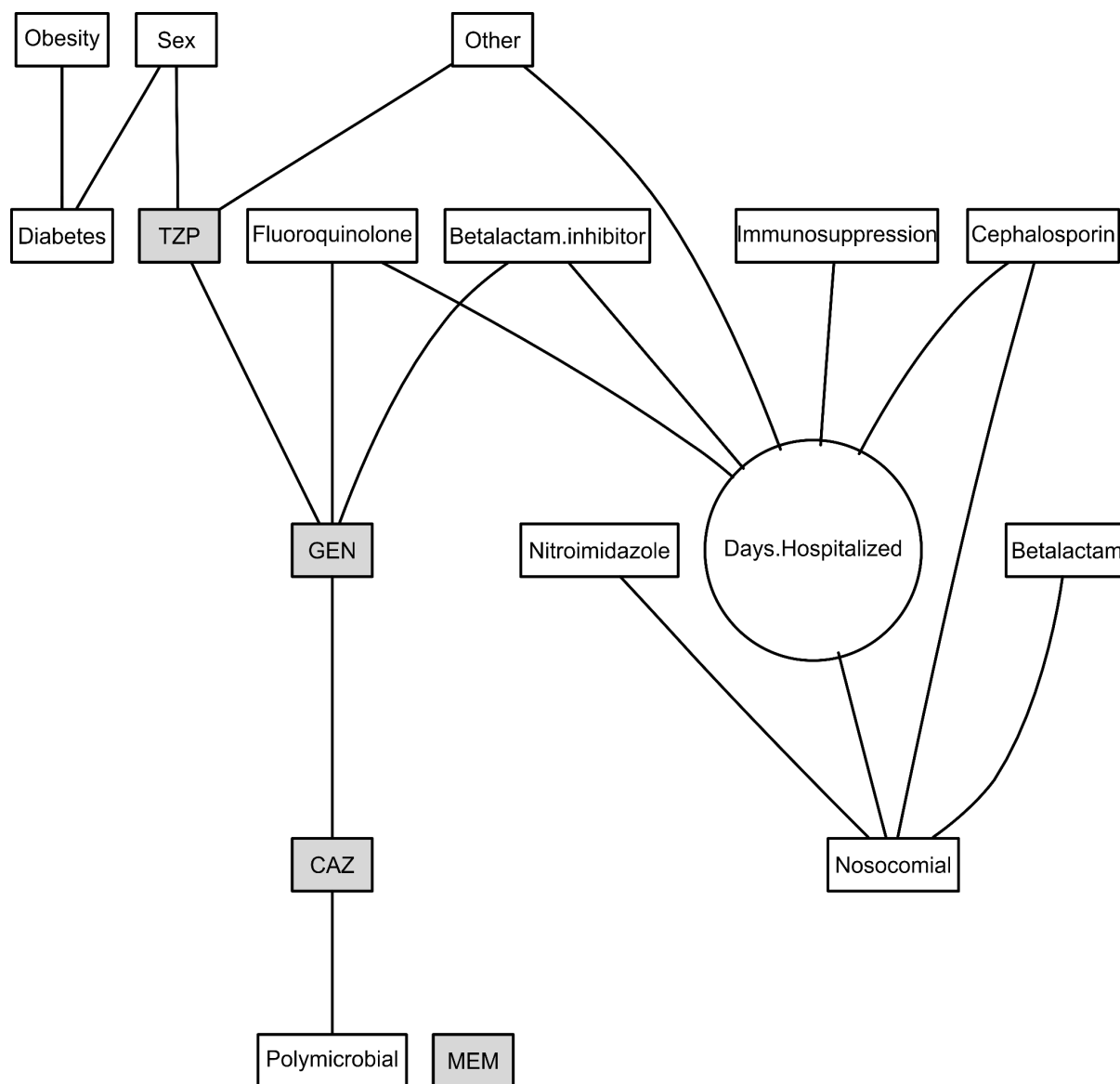
Figure 1: Additive Bayesian network for P. aeruginosa in wound samples. Variables in rectangles are binary and the one in a circle is continuous. Drug family variables refer to a particular drug taken in the prior year. Antibiotic resistance tests are shown in shaded boxes: CAZ, ceftazidime; GEN, gentamicin; MEM, meropenem, TZP, piperacillin/tazobactam.
