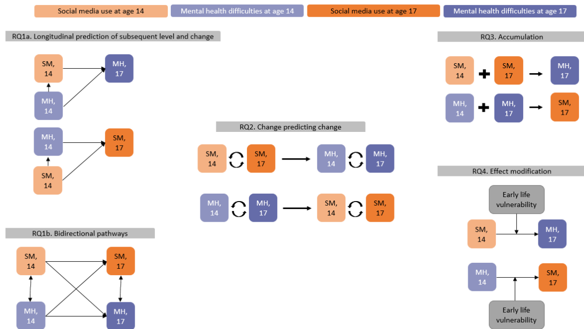
Figure 1. Schematic overview of the RQs and the models estimated to answer each.
