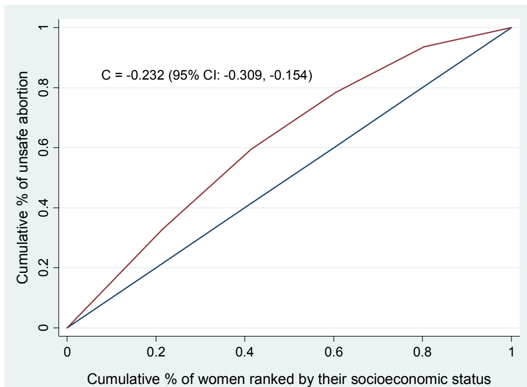
Figure 1: Concentration curve for cumulative proportion of unsafe abortion ranked by wealth index among women who presented for abortion care services in public hospitals in 2020, Lusaka and Copperbelt provinces, Zambia
