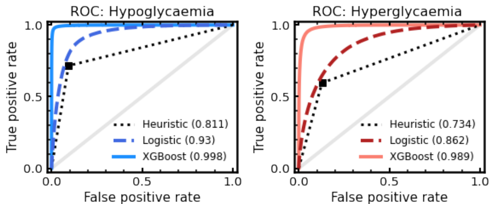
Figure 2: Receiving operator characteristic (ROC) for our models of hypoglycaemia (left) and hyperglycaemia (right) prediction. In each panel, a XGBoost model (solid line) and a logistic regression model (dashed line) are compared to a baseline heuristic (dotted line). A zero skill model is represented by the solid grey line. The total area under each curve (i.e. AUROC score) is given in the brackets.
