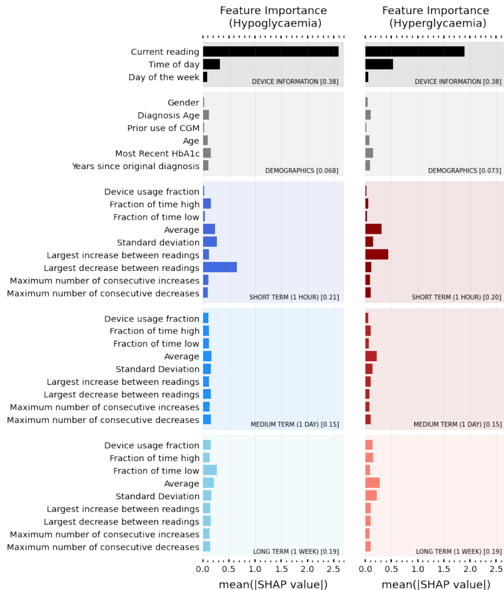
Figure 3: Overall importance ranking of input features for predicting hypo (left panel) and hyper (right panel) risk. Average (absolute) SHAP value for predictive features over all study participants. A higher value corresponds to a more important feature in decision making. Features are grouped into categories (Device information, Demographics, Short term (1 hour), Medium Term (1 day), Long term (1 week)). The fractional contribution (i.e. sum over all features in that category) of a given category is given in the square brackets.
