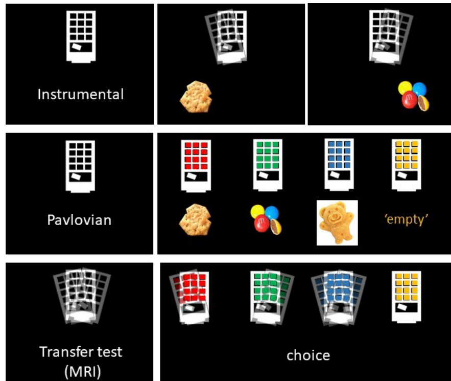
Figure 1. Pavlovian-instrumental transfer.
