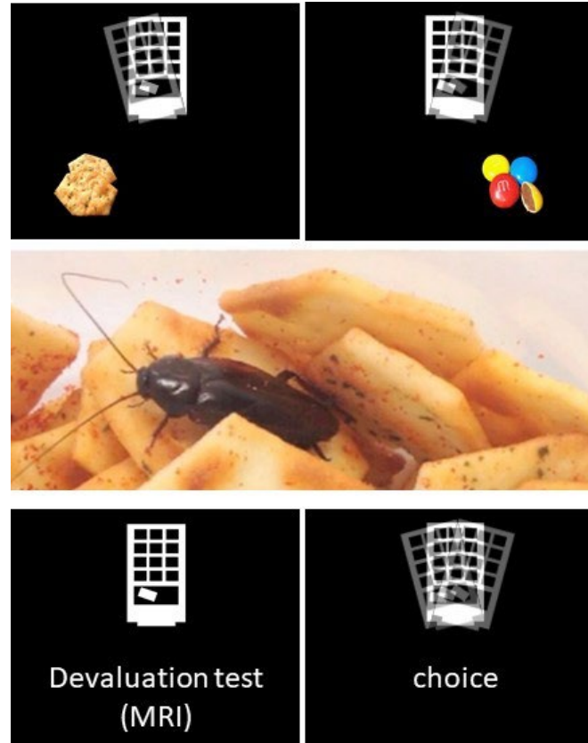
Figure 3. Outcome devaluation
