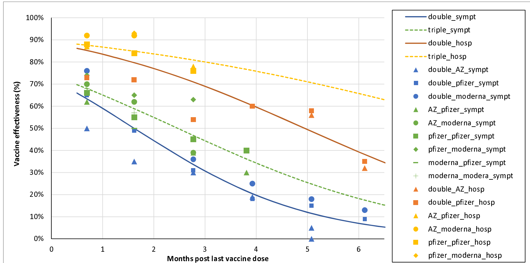
Figure 1: Predicted vaccine effectiveness against the Omicron SARS-CoV-2 variant using a log-odds system, overlaid with observed data points used to fit model
