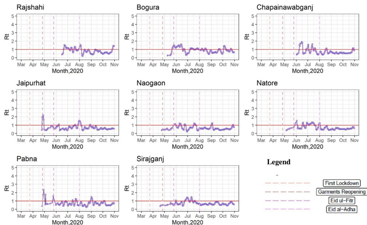
S3 Fig: Dynamics of R_t values over time (March, 2020 – October, 2020) in Rajshahi Division
