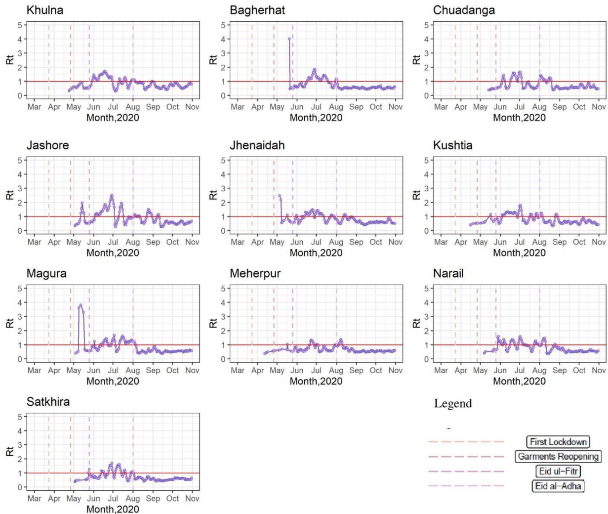
S5 Fig: Dynamics of R_t values over time (March, 2020 – October, 2020) in Khulna Division
