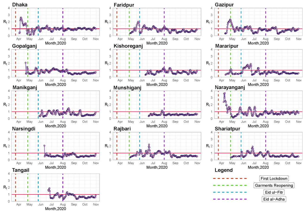
Fig 2. Comprehensive analysis of R_t values over time (March, 2020 – October, 2020) in Dhaka Division
