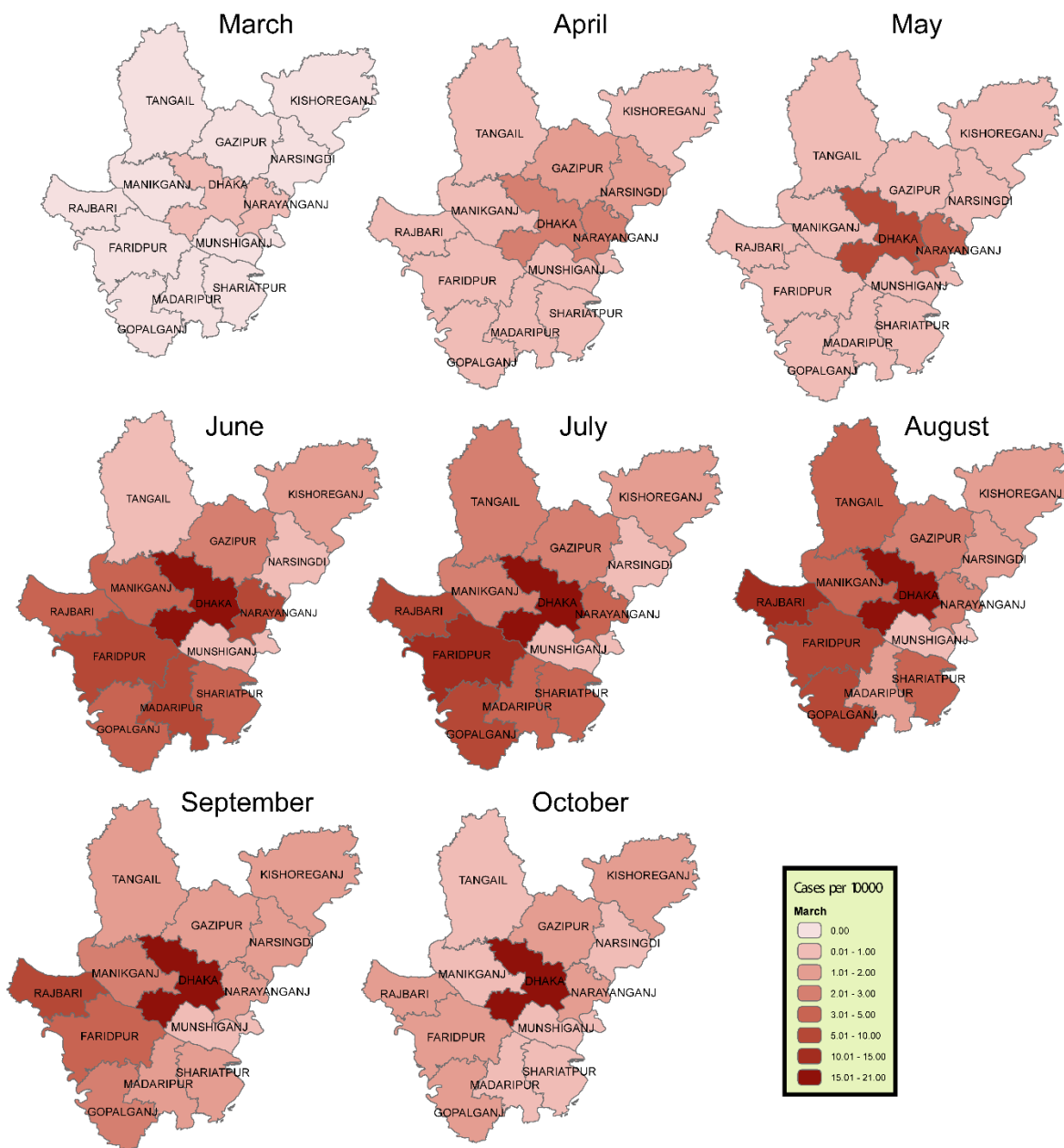
Fig 1. Propagation of COVID-19 from March, 2020 to October, 2020 in Dhaka Division
