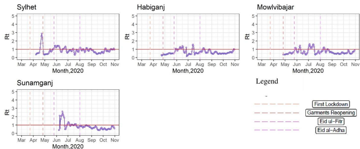
S2 Fig: Dynamics of R_t values over time (March, 2020 – October, 2020) in Sylhet Division
