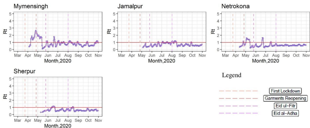
S1 Fig Dynamics of R_t values over time (March, 2020 – October, 2020) in Mymensingh Division
