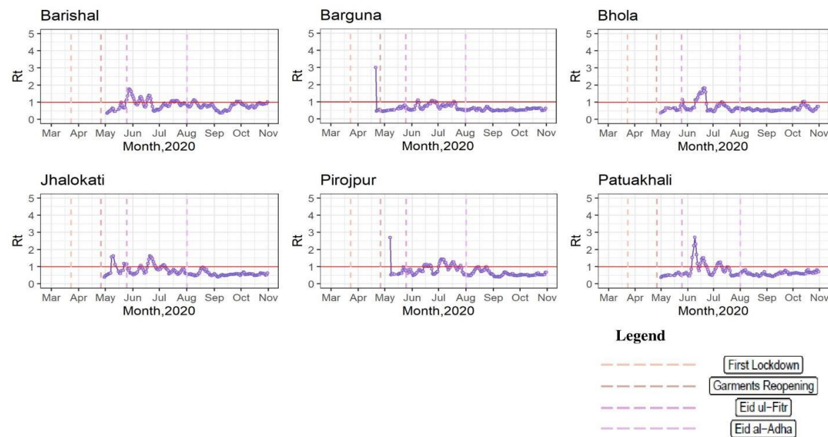
S4 Fig: Dynamics of R_t values over time (March, 2020 – October, 2020) in Barishal Division
