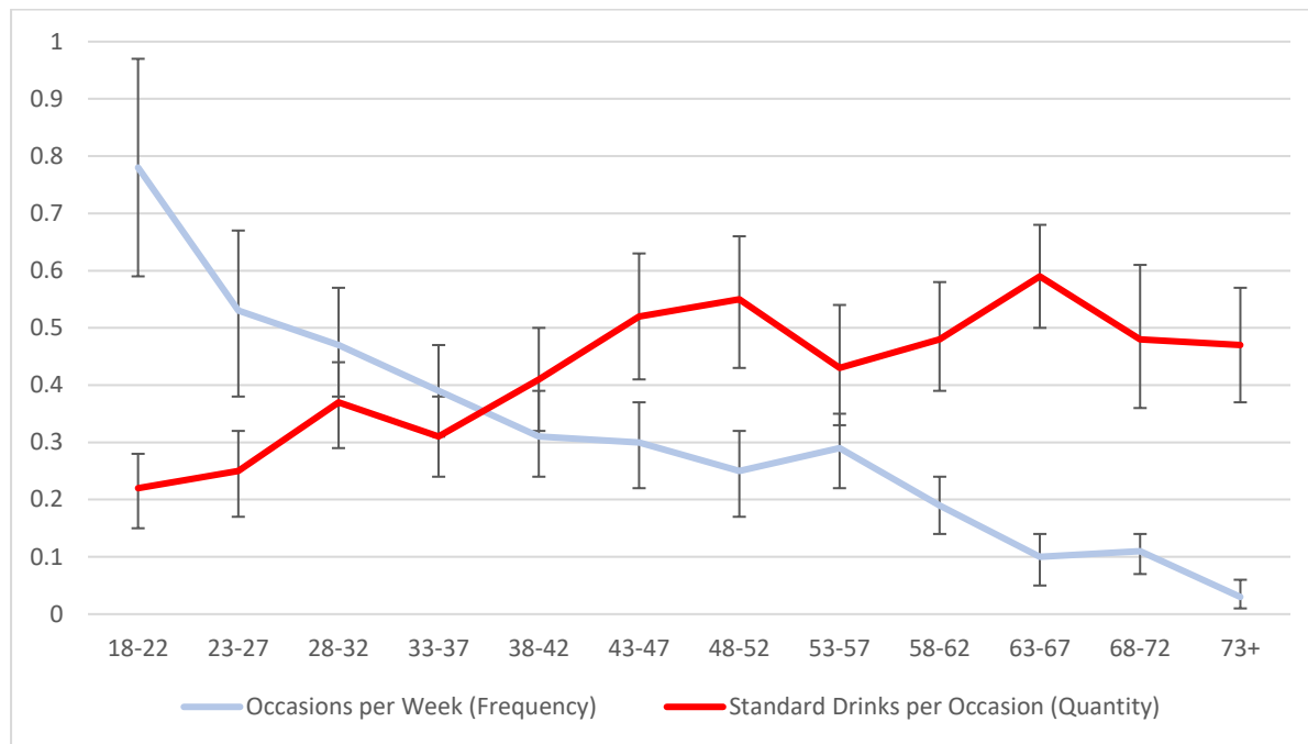
Figure 3. Beta coefficients of standardised usual quantity and frequency of drinking as predictors of the AUDIT harmful drinking subscale.
