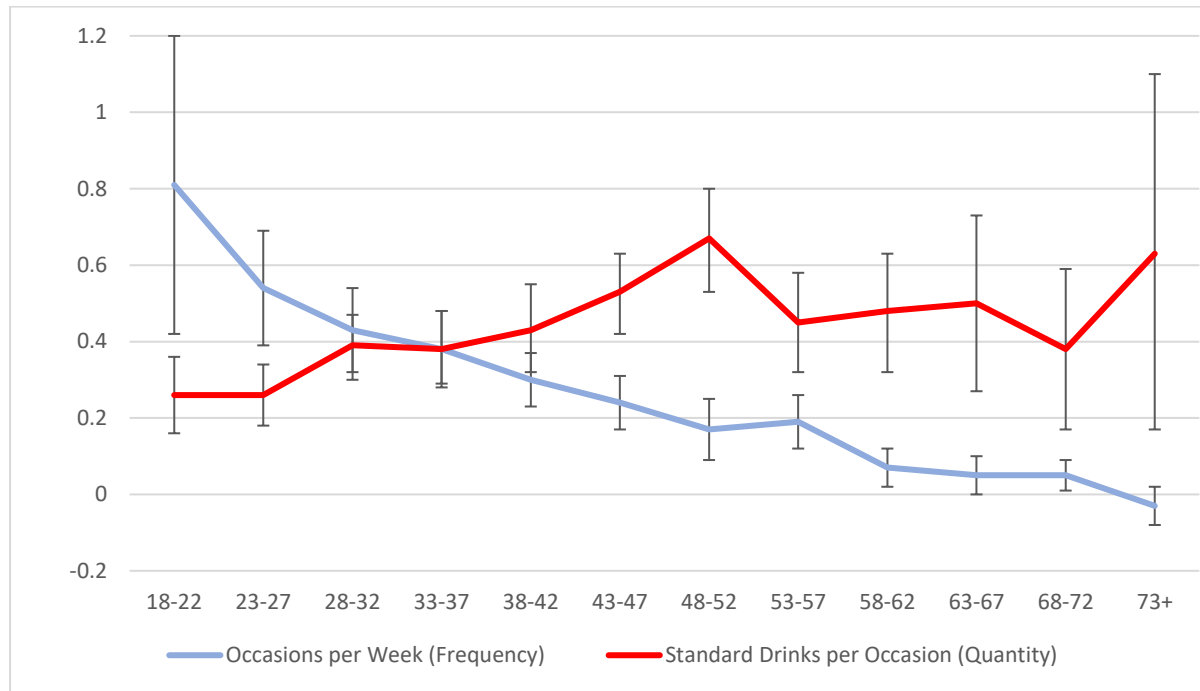
Figure 2. Beta coefficients of standardised usual quantity and frequency of drinking as predictors of the AUDIT dependence subscale.
