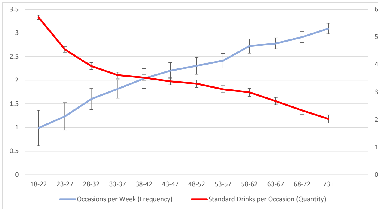
Figure 1: Average number of drinking occasions per week (frequency, left scale) and number of standard drinks per usual occasion (quantity, right scale), with 95% confidence intervals, by age
