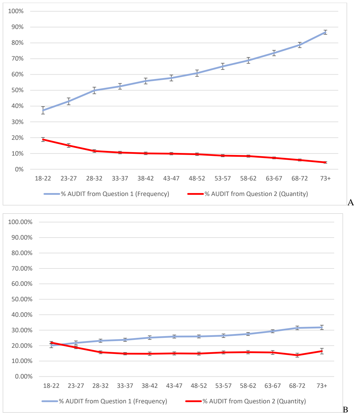
Figure 4. Proportion of the full AUDIT score that can be attributed to the question on frequency (item 1) and usual quantity (item 2). Panel A includes all participants, Panel B includes only those who had a total AUDIT score of 8 or more.
