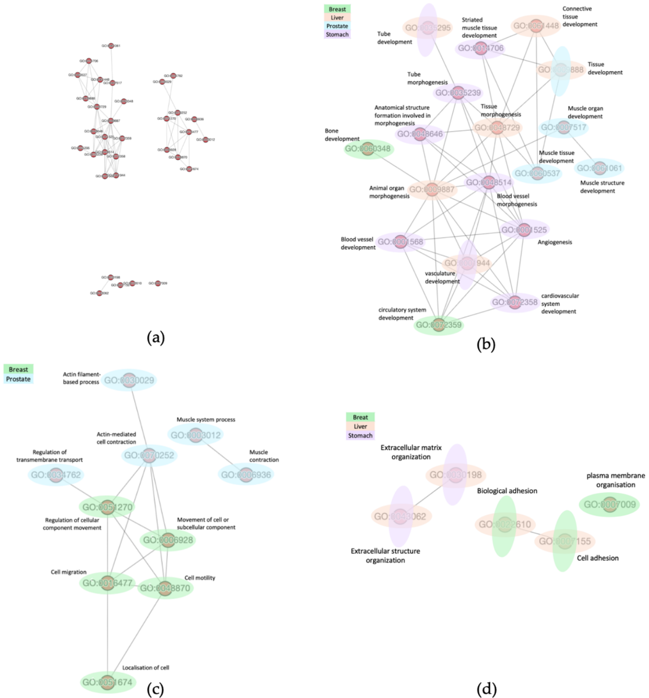
Figure 4. Functional similarity of GO terms associated with mRNAs of positive correlation with lncRNA Antisense. Network visualisation of functional similarity of GO terms enriched by positively correlated mRNAs with lncRNA "Antisense", across cancers (when applicable, RSS \geq 0.05). (a) Three clusters can be visually identified. (b) Close up of cluster 1. (c) Close up of cluster 2 (d) Close up of cluster 3. (b) , (c) and (d) : Each node indicates a GO term and the edges (lines in between) represent a functional similarity, representing relationships, such as "is a" or "part of". The colour(s) of nodes represent the cancer type(s) in which GO term was found to be enriched, green for breast cancer (BRCA), orange for liver cancer (LIHC), blue for prostate cancer (PRAD) and purple for stomach cancer (STAD).
