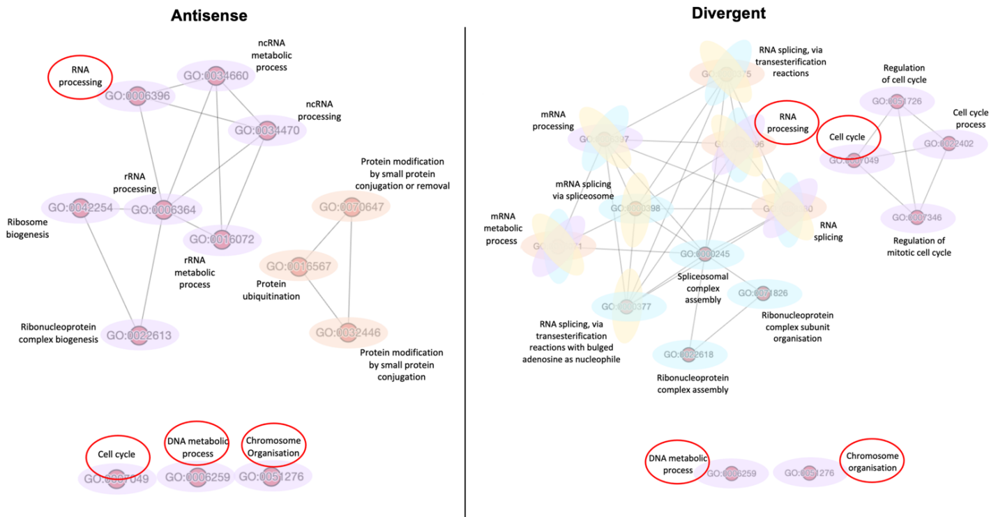
Figure 8. Comparison of Antisense and Divergent GO terms similarity networks. Similarity networks among GO terms enriched by mRNAs related negatively to Antisense (left) and mRNAs related positively to Divergent (right). Shared GO terms in both networks are encircled in red.
