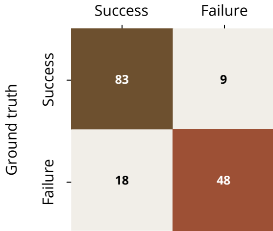
Figure 7a. ABNN's performance in terms of confusion matrices for all therapeutic areas.
