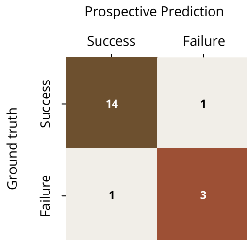
Figure 7c. ABNN's performance in terms of confusion matrices per therapeutic area.
